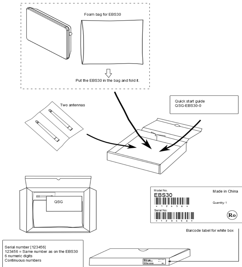
Figure 4: Individual Packing
