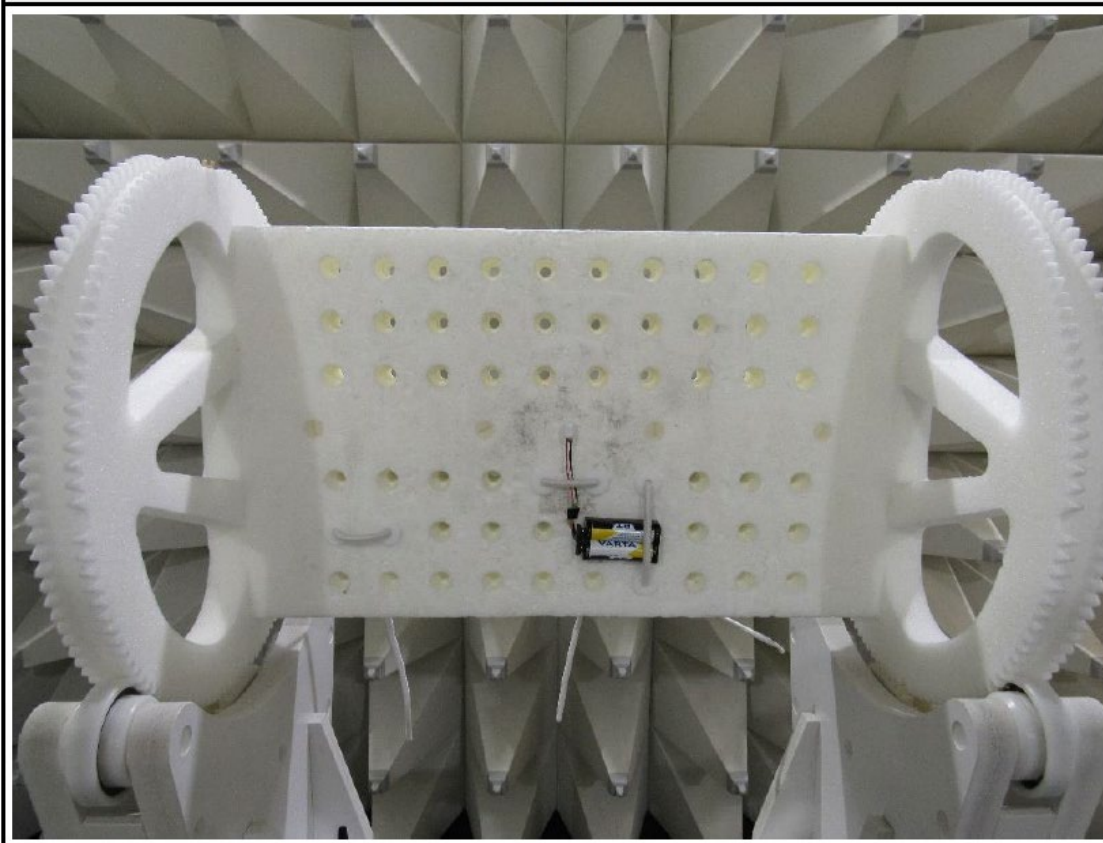
EUT test setup above 1 GHz
