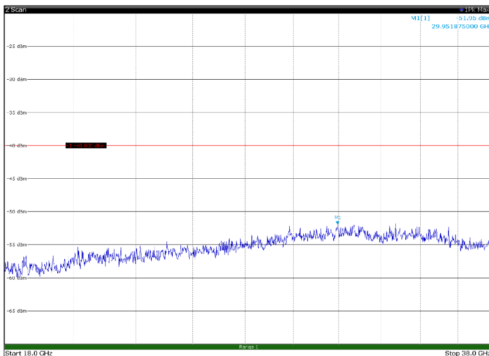
Channel: BOTTOM, Modulation: 64QAM, BW=5MHz, Range: 18GHz - 38GHz, Polarization: Vertical
