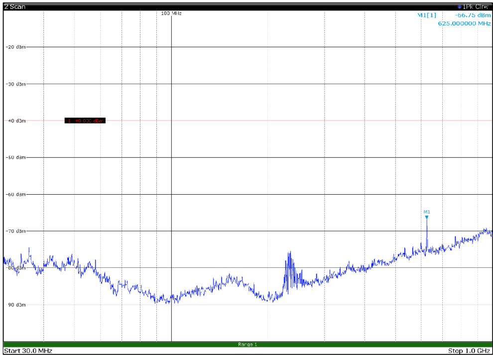
Channel: MIDDLE, Modulation: 16QAM, BW=5MHz, Range: 30MHz - 1GHz, Polarization: Horizontal
