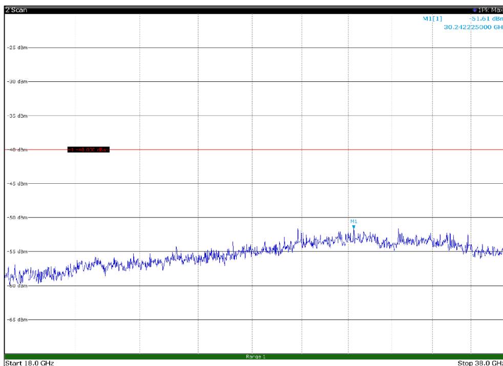
Channel: MIDDLE, Modulation: 64QAM, BW=5MHz, Range: 18GHz - 38GHz, Polarization: Vertical
