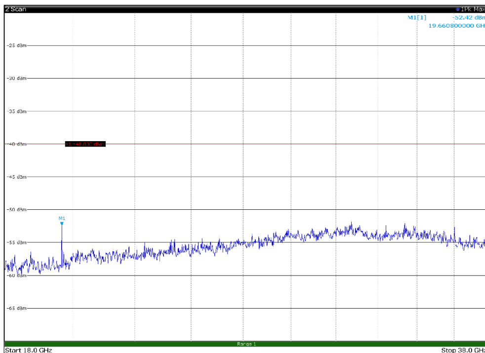
Channel: BOTTOM, Modulation: 64QAM, BW=5MHz, Range: 18GHz - 38GHz, Polarization: Horizontal
