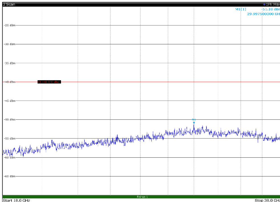
Channel: MIDDLE, Modulation: 16QAM, BW=5MHz, Range: 18GHz - 38GHz, Polarization: Vertical
