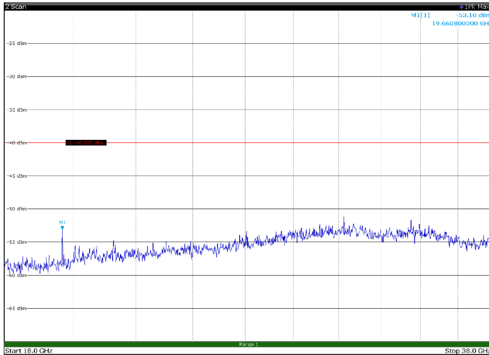
Channel: MIDDLE, Modulation: 16QAM, BW=5MHz, Range: 18GHz - 38GHz, Polarization: Horizontal
