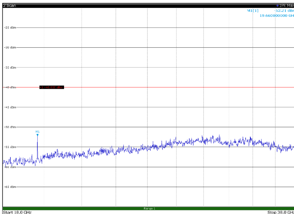
Channel: MIDDLE, Modulation: 64QAM, BW=5MHz, Range: 18GHz - 38GHz, Polarization: Horizontal
