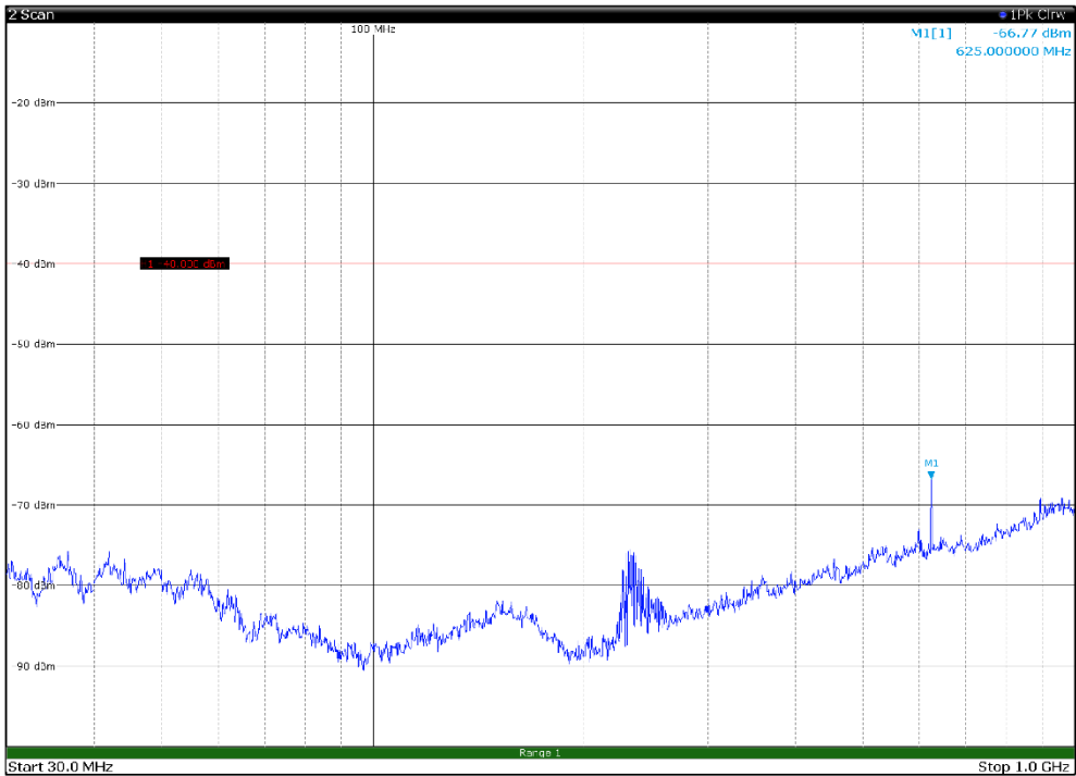
Channel: BOTTOM, Modulation: QPSK, BW=5MHz, Range: 30MHz - 1GHz, Polarization: Horizontal
