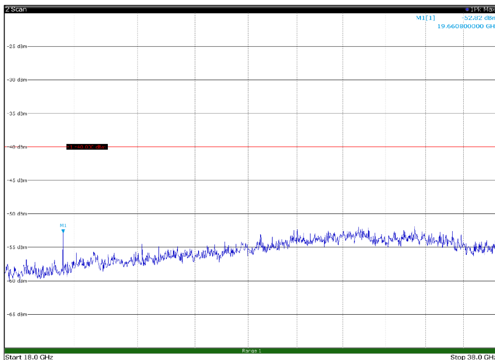
Channel: TOP, Modulation: 256QAM, BW=5MHz, Range: 18GHz - 38GHz, Polarization: Horizontal
