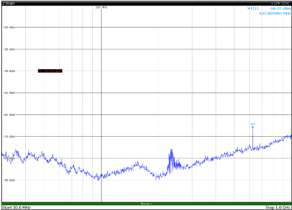
Channel: MIDDLE, Modulation: 256QAM, BW=5MHz, Range: 30MHz - 1GHz, Polarization: Horizontal
