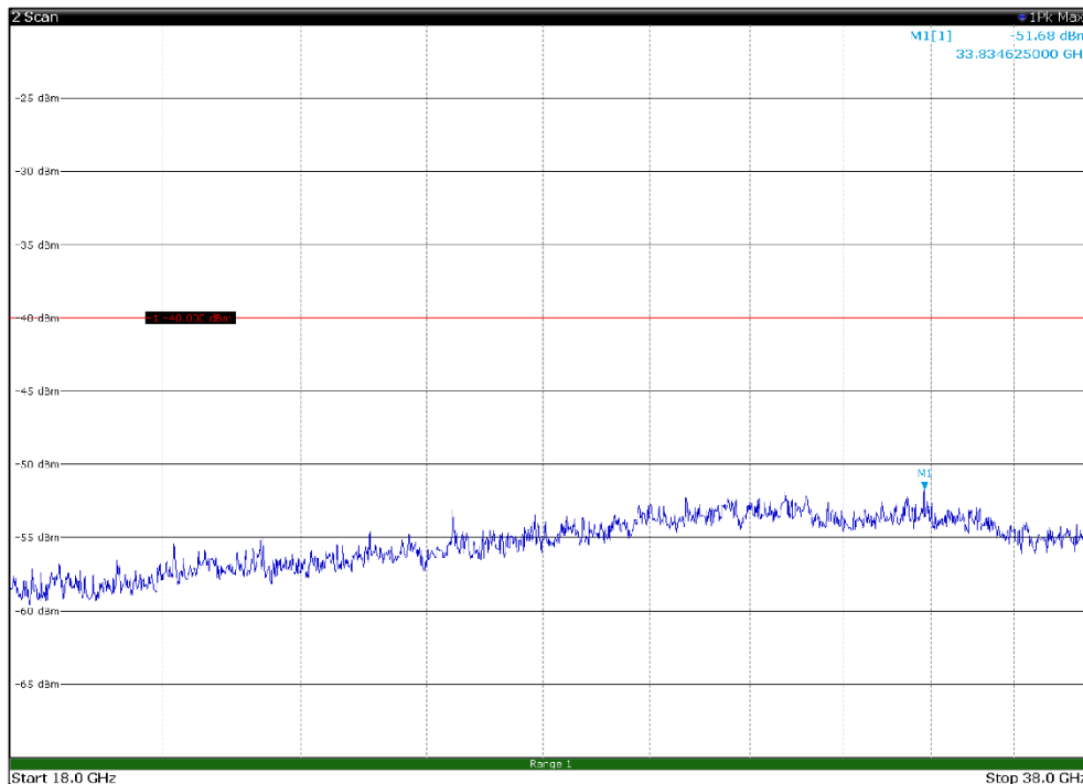
Channel: TOP, Modulation: 64QAM, BW=5MHz, Range: 18GHz - 38GHz, Polarization: Vertical
