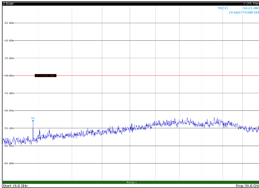
Channel: TOP, Modulation: 64QAM, BW=5MHz, Range: 18GHz - 38GHz, Polarization: Horizontal
