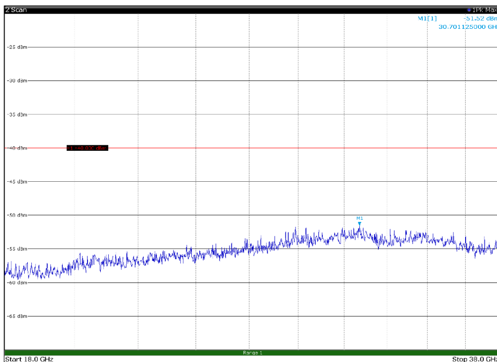
Channel: TOP, Modulation: 256QAM, BW=5MHz, Range: 18GHz - 38GHz, Polarization: Vertical
