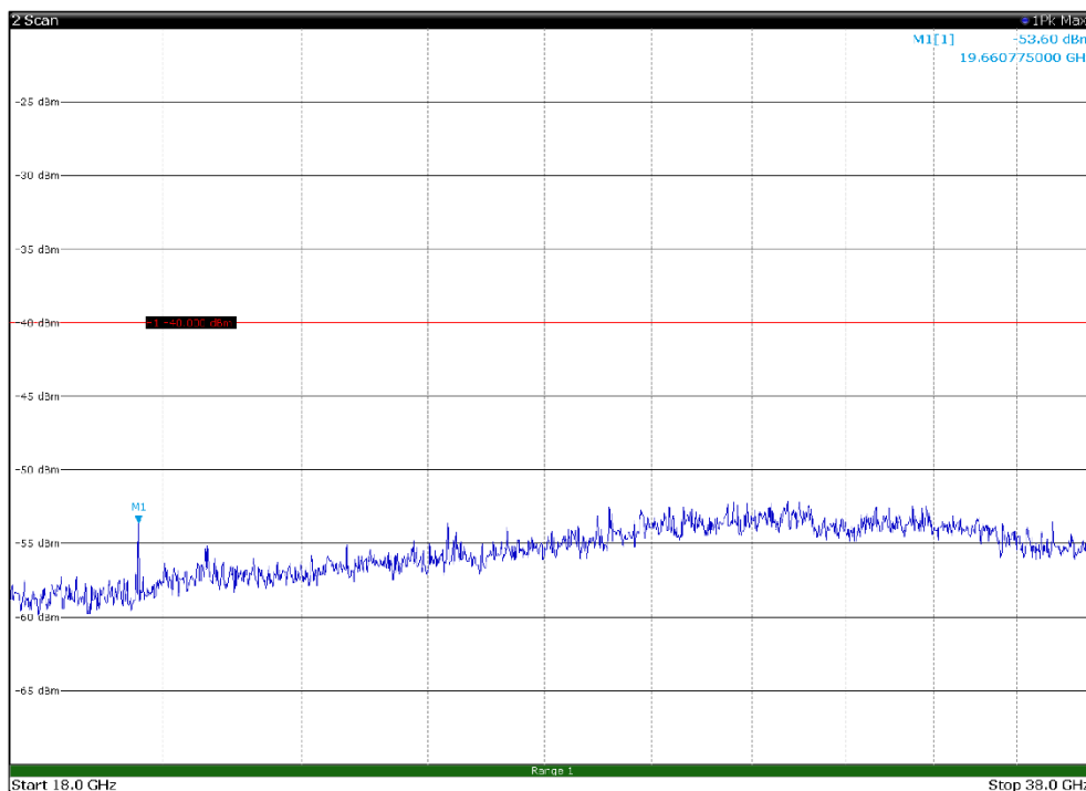
Channel: MIDDLE, Modulation: QPSK, BW=5MHz, Range: 18GHz - 38GHz, Polarization: Horizontal
