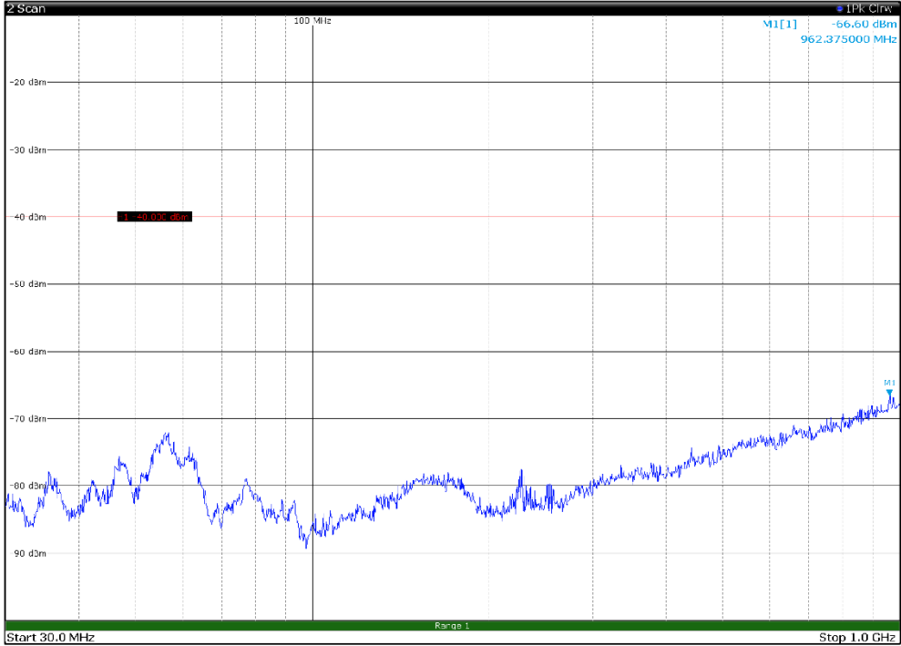
Channel: MIDDLE, Modulation: 256QAM, BW=5MHz, Range: 30MHz - 1GHz, Polarization: Vertical
