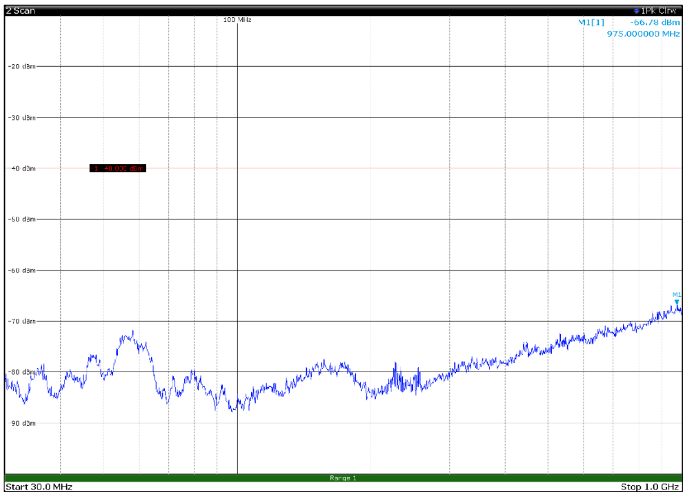
Channel: MIDDLE, Modulation: 16QAM, BW=5MHz, Range: 30MHz - 1GHz, Polarization: Vertical
