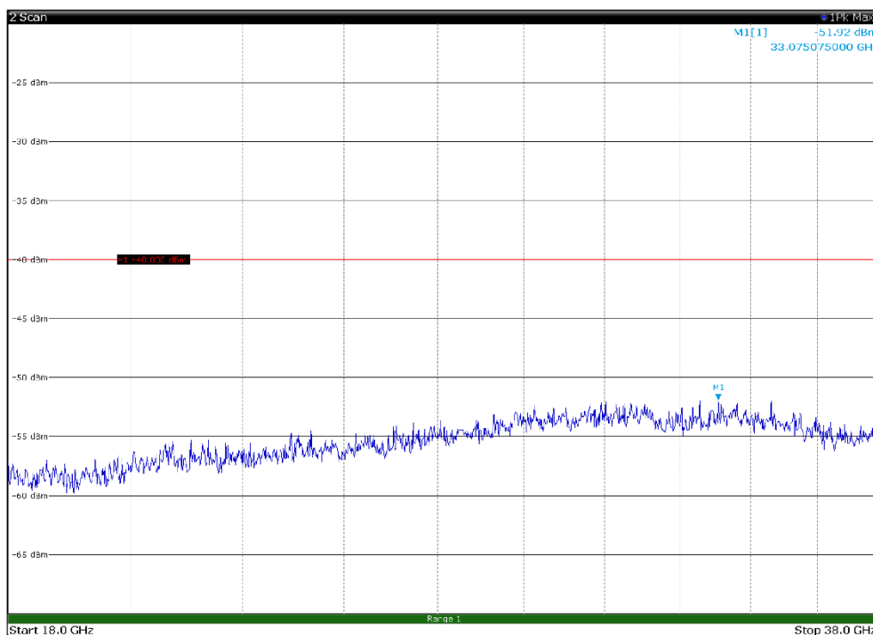
Channel: MIDDLE, Modulation: QPSK, BW=5MHz, Range: 18GHz - 38GHz, Polarization: Vertical
