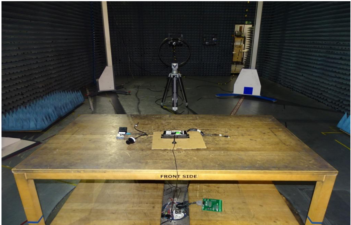
Photo 1: Test setup for radiated measurements below 30 MHz
