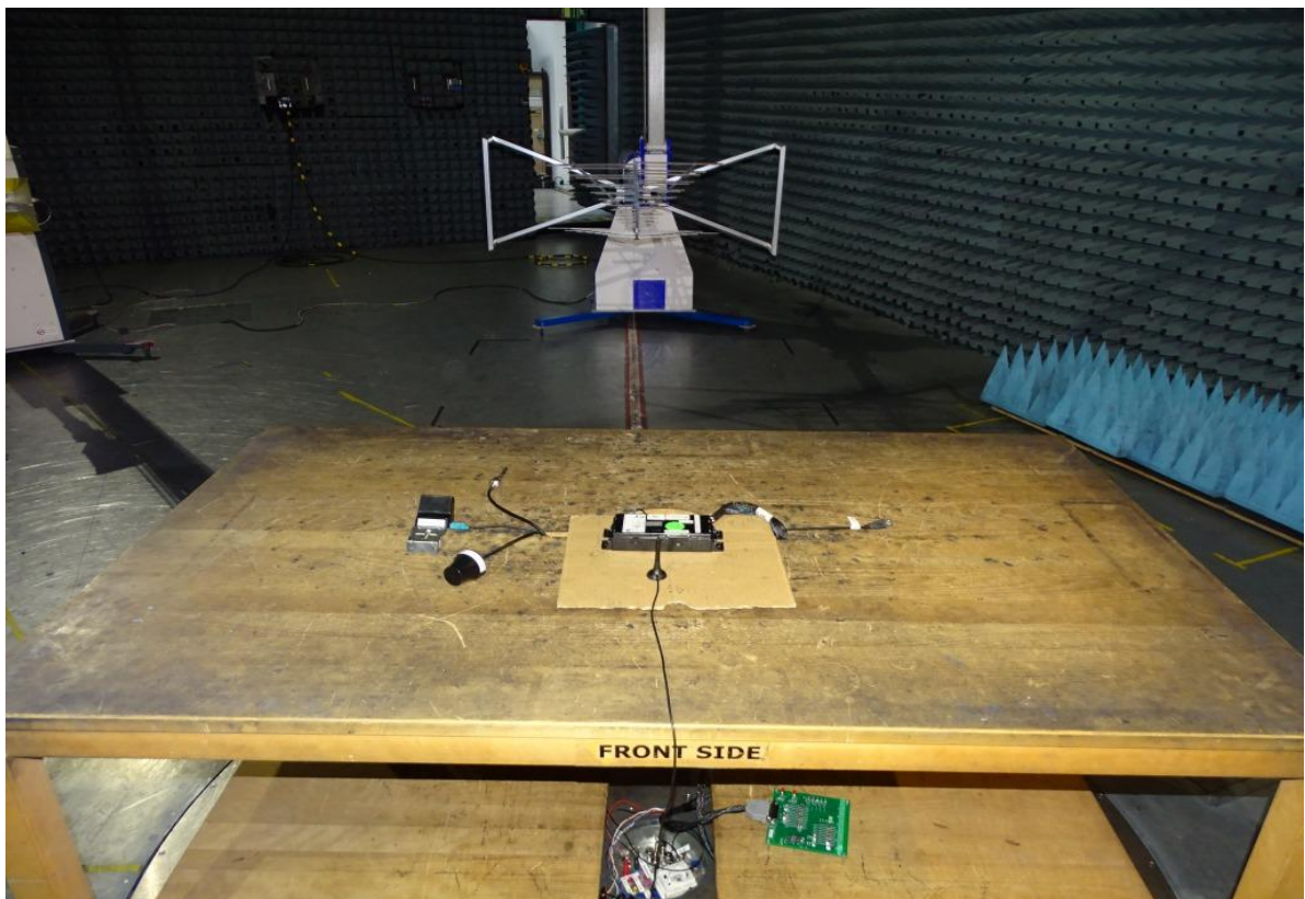
Photo 2: Test setup for radiated measurements below 1 GHz
