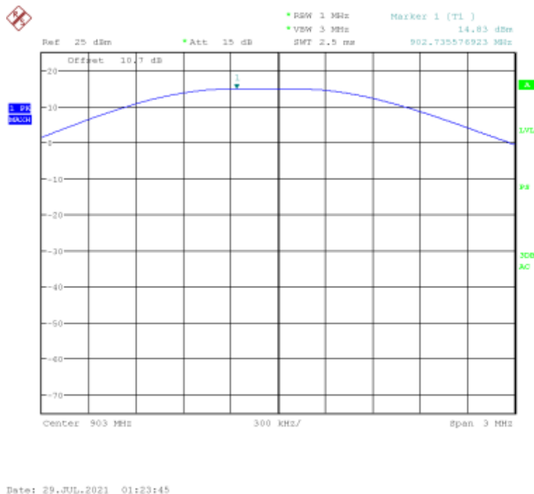
Figure 4 – Low Channel Output Power (FSK)
