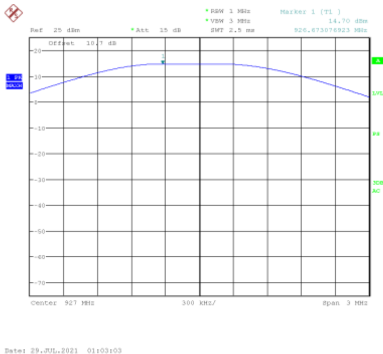
Figure 3 – High Channel Output Power (LoRa)
