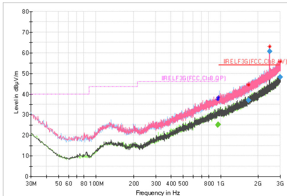
Plot 7: Radiated Emissions scanned at 3m SAC
