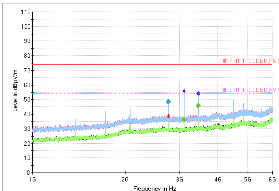
Plot 6: Radiated Emissions (1GHz-6GHz) scanned at 3m SAC
