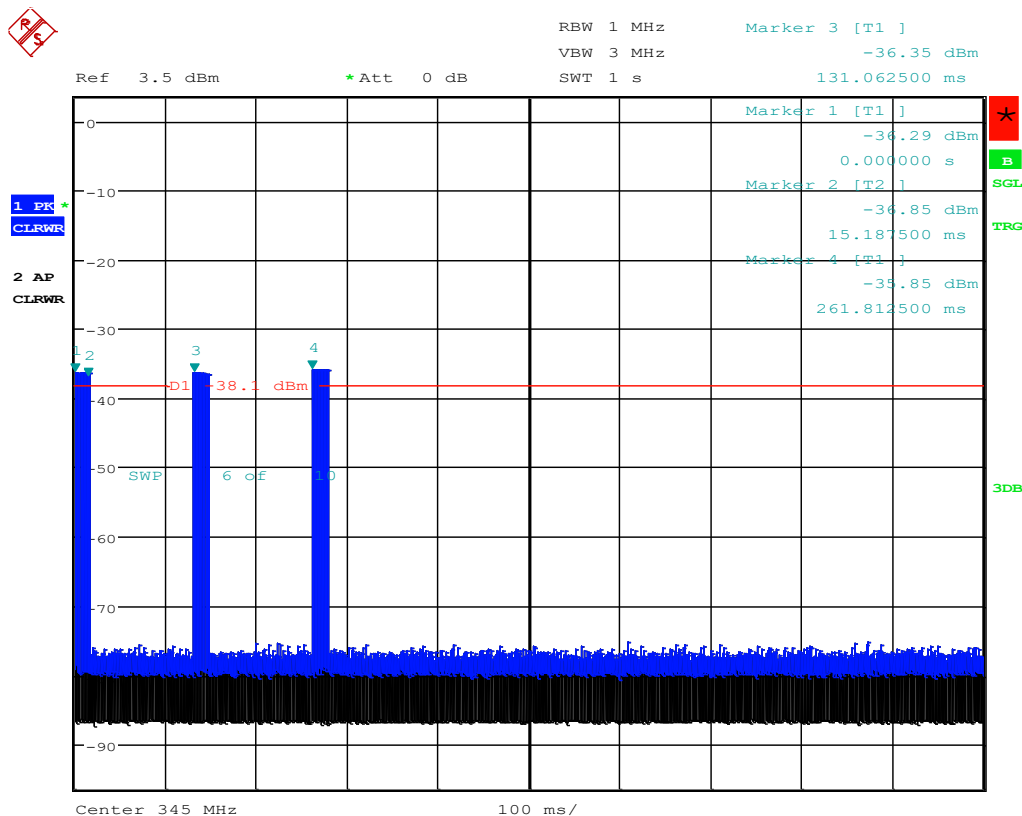
Plot 1: Transmission Time Measurement
