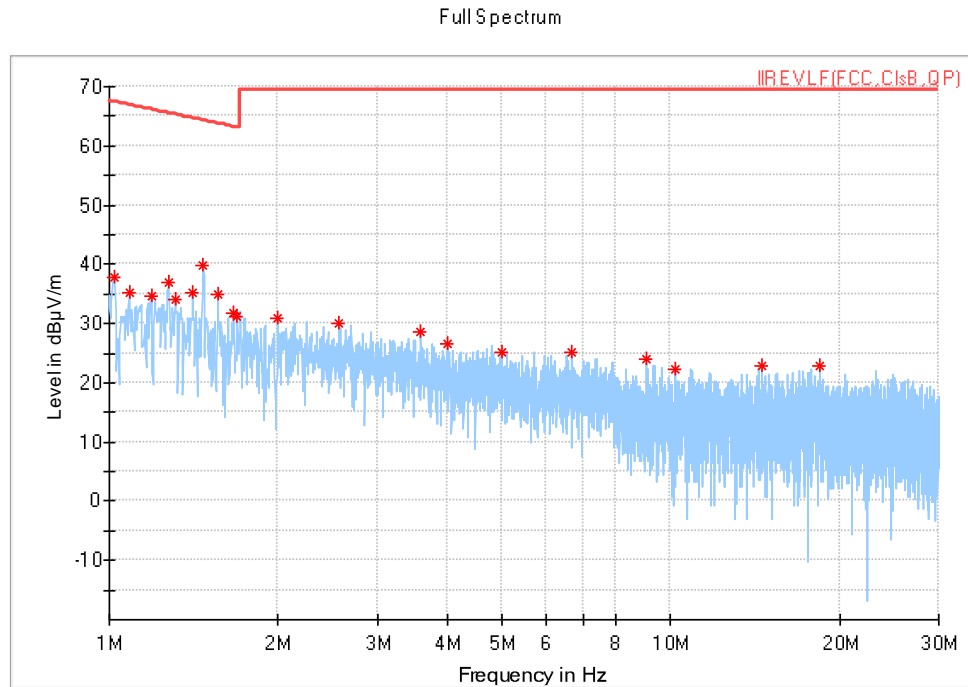
Plot 4: Radiated Emissions (1-30M Hz) – Parallel Pol.
