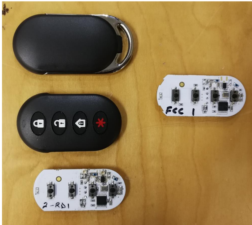
EUT – KF2GIG: Casing, normal operation and CW units
