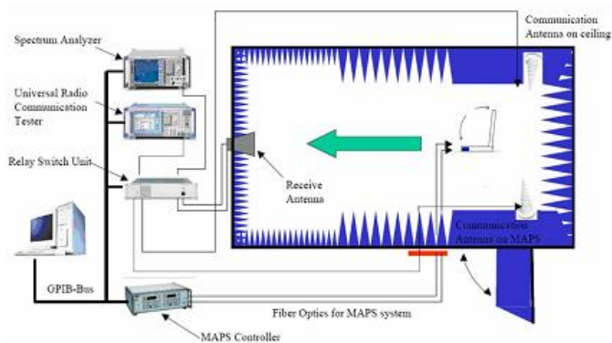
(Testing by 3D anechoo chamber)
