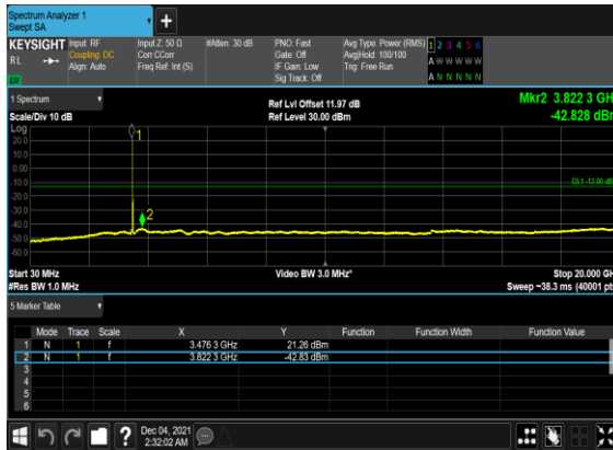
B41_N77(50M)_DFT-s-OFDM_QPSK_Edge_1RB_Left_Mid_CH
