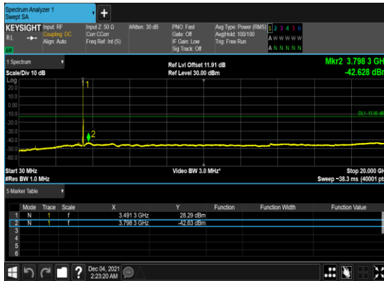
B41_N77(20M)_DFT-s-OFDM_QPSK_Edge_1RB_Left_Mid_CH
