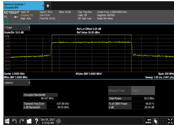
B41_N77(100M)_DFT-s- OFDM_QPSK_Outer_Full_Mid_CH
