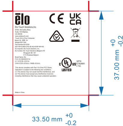
ESY1514,AOSP SAFETY LABEL Artwork for Label Manufacture-White SCALE 1:1 OUTLINE
