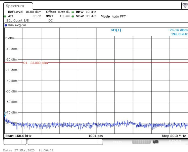
Band5-5MHz-QPSK-20425-1RB#0-Range3:30~1000MHz
