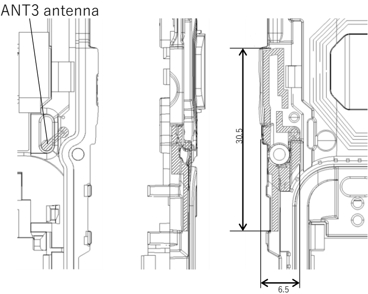
External view of antenna (Bluetooth/WLAN antenna)
