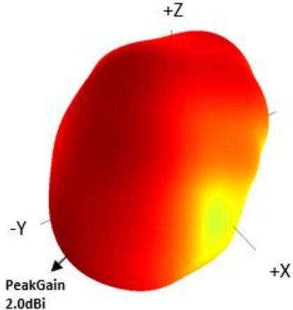
ANT5 WLAN6G
