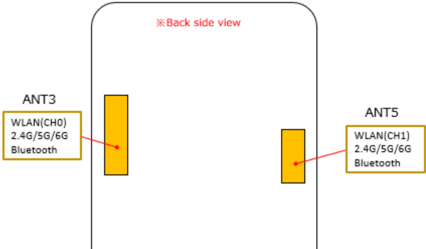
External view of antenna (Bluetooth/WLAN antenna)
