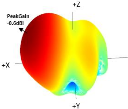
ANT5 WLAN5G
