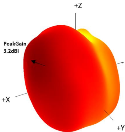
ANT3 WLAN6G
