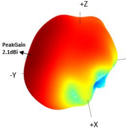
ANT5 WLAN6G
