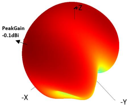
ANT3 WLAN5G
