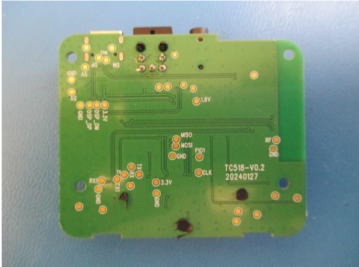
PC Board Bottom Side
