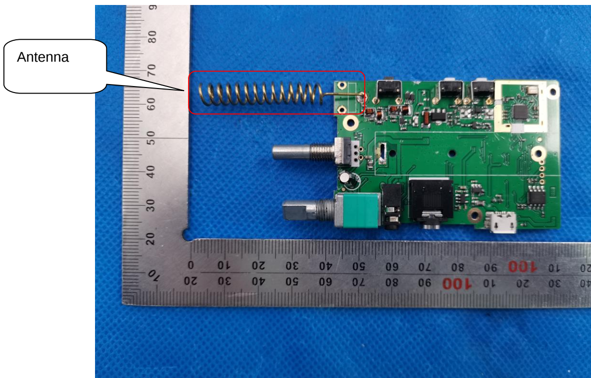
INTERNAL VIEW OF EUT (FIGURE 2)
