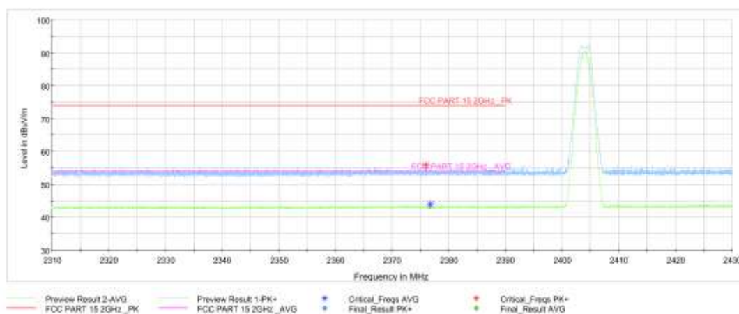
Fig.18. Frequency Band Edges: GFSK, 2404 MHz, Hopping Off, 2.31 GHz – 2.43GHz
