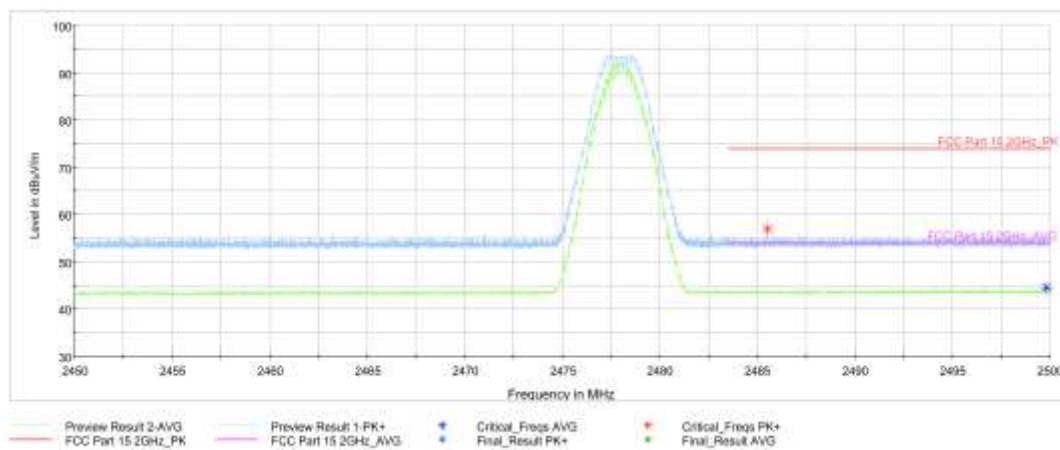
Fig.19. Frequency Band Edges: GFSK, 2478 MHz, Hopping Off, 2.45 GHz - 2.50GHz
