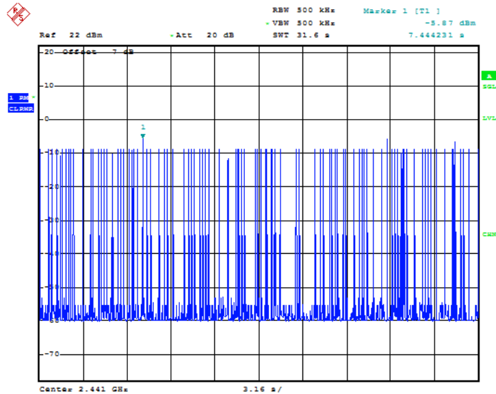
Fig.70 Time of occupancy (Dwell Time): Ch39, Packet 2-DH5
