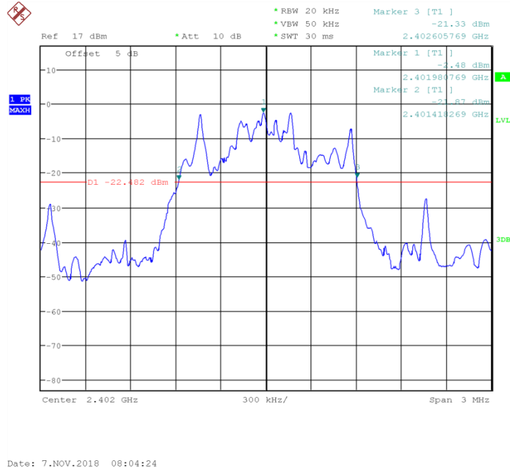
Fig.84 20dB Bandwidth: 8DPSK, Ch0
