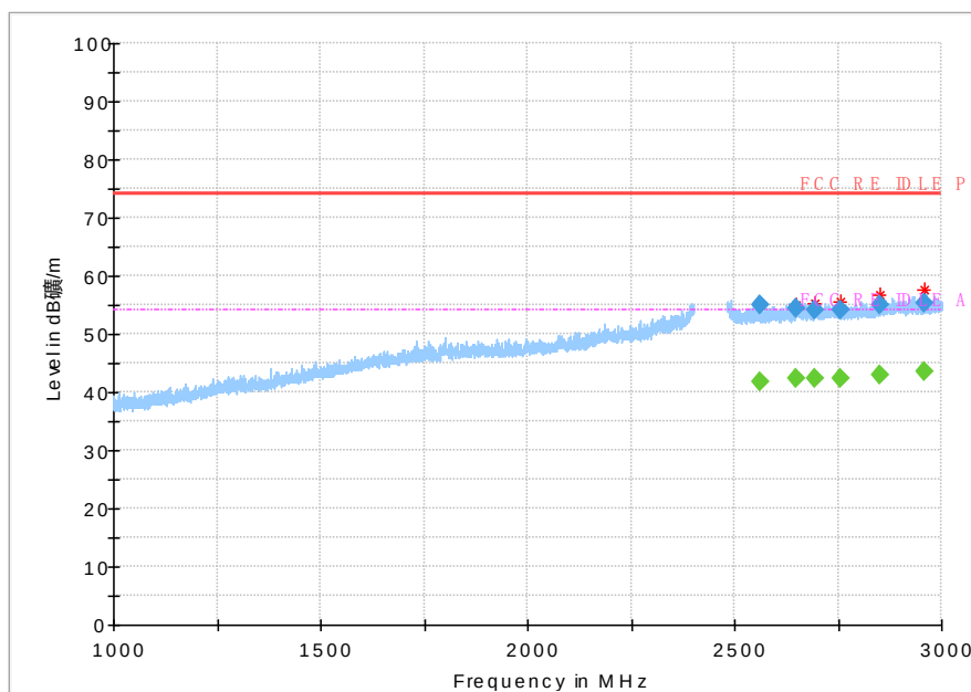
Fig.56 Radiated emission: GFSK, Ch78, 1GHz~3GHz
