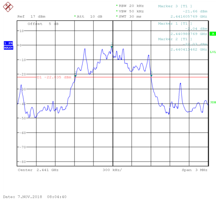
Fig.85 20dB Bandwidth: 8DPSK, Ch39
