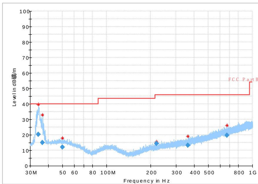
Fig.55 Radiated emission: GFSK, Ch78, 30MHz~1GHz
