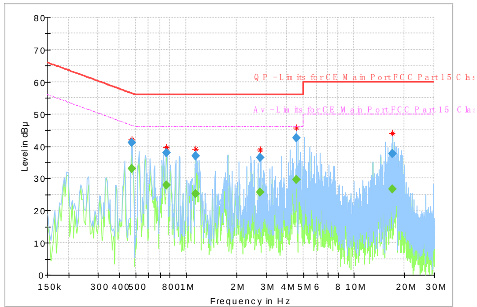
Fig.96 AC Powerline Conducted Emission
