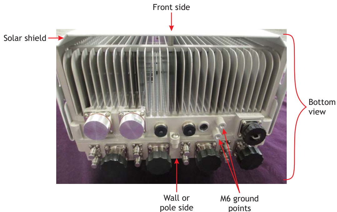
Figure 3-2 Alcatel-Lucent B25 RRH4x30 grounding points
