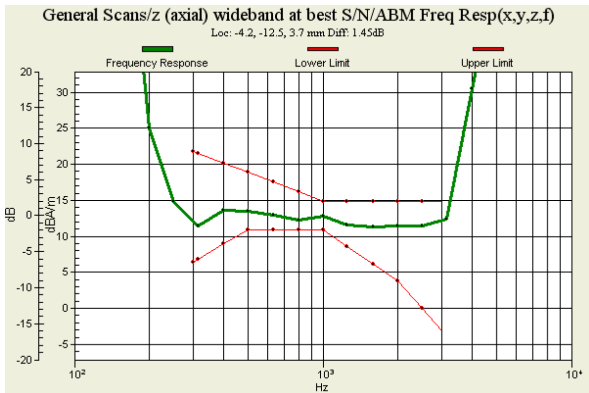
Figure 20 T-Coil WCDMA Band V Z Axial
