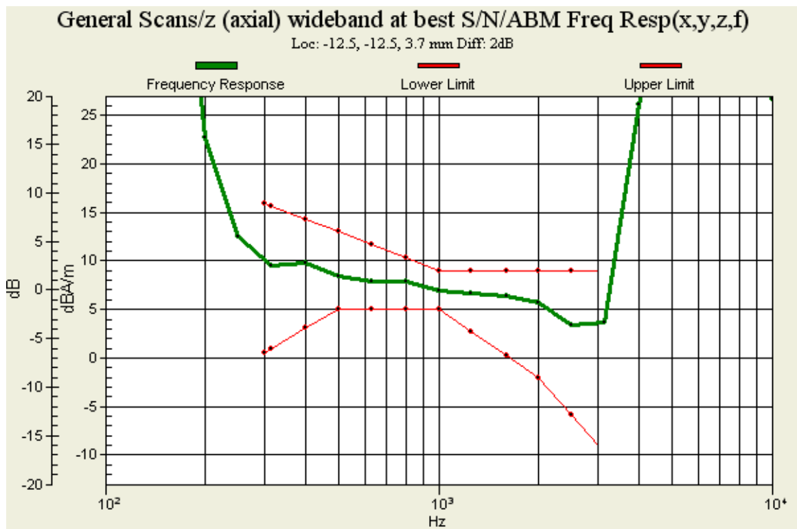
Figure 12 T-Coil GSM 850 Z Axial
