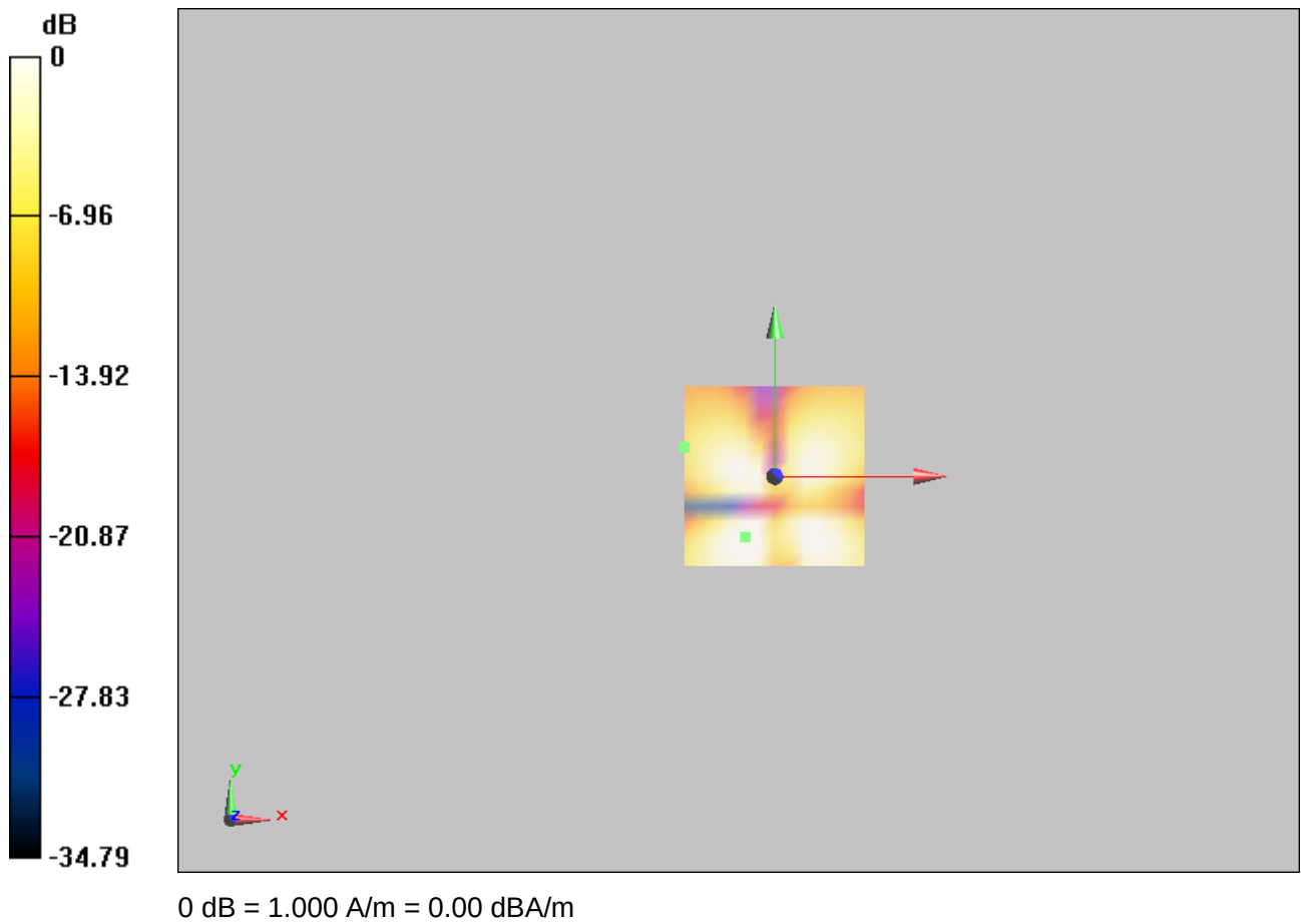
Figure 13 T-Coil GSM 1900 Y transversal
