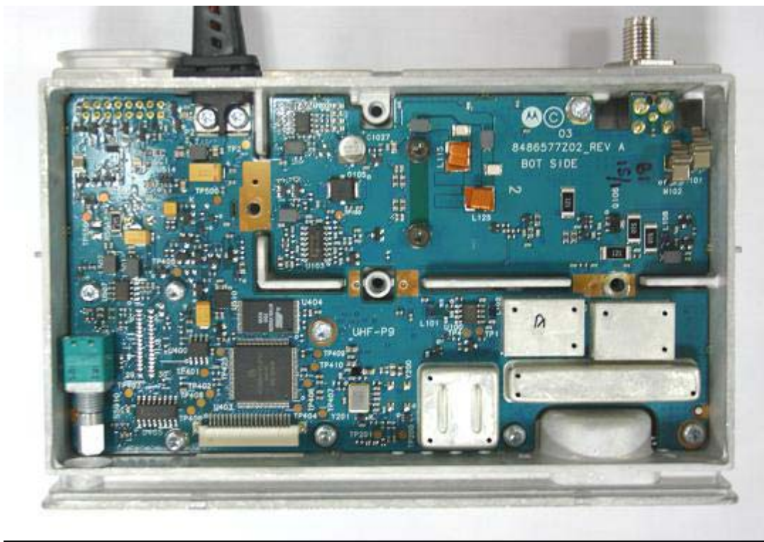
Figure 9-5: Top View of PCB placed in chassis.
