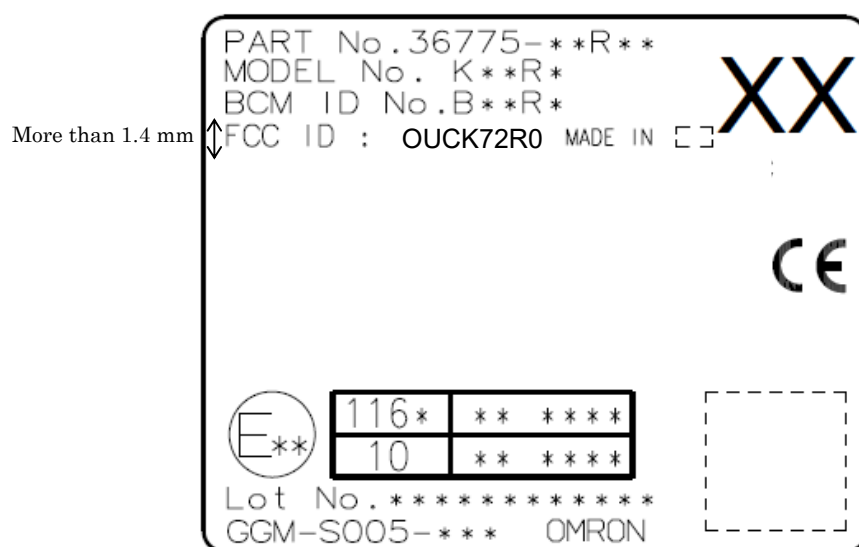
Figure 9.1 K72R0 Label
