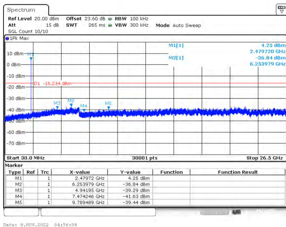
Tx. Spurious NVNT 3-DH1 2480MHz Ant1 Emission
