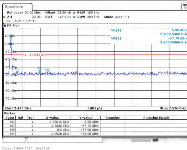
No-hopping mode
