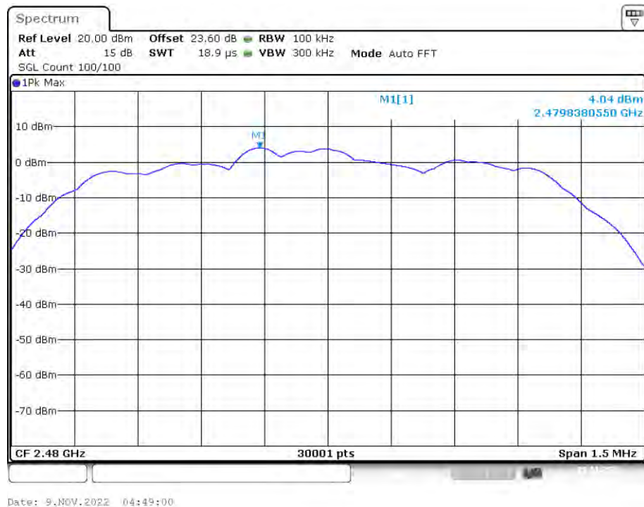
Tx. Spurious NVNT 2-DH1 2480MHz Ant1 Emission
