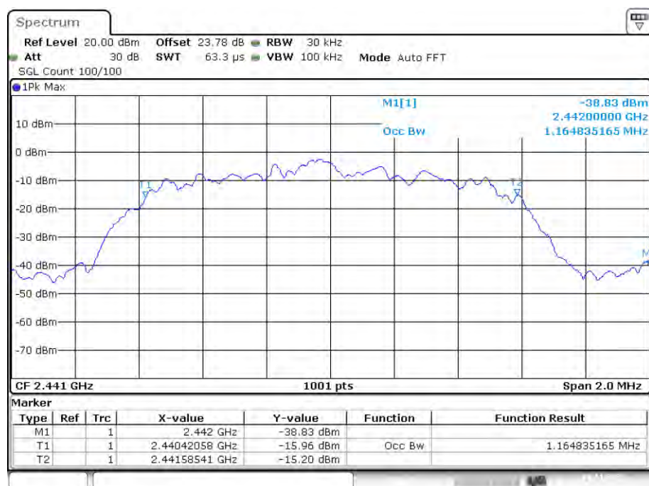
OBW NVNT 3-DH1 2441MHz Ant1
