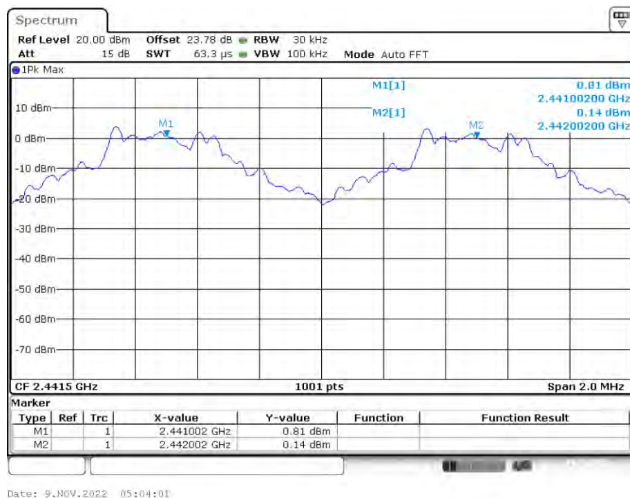
CFS NVNT 2-DH1 2441MHz Ant1
