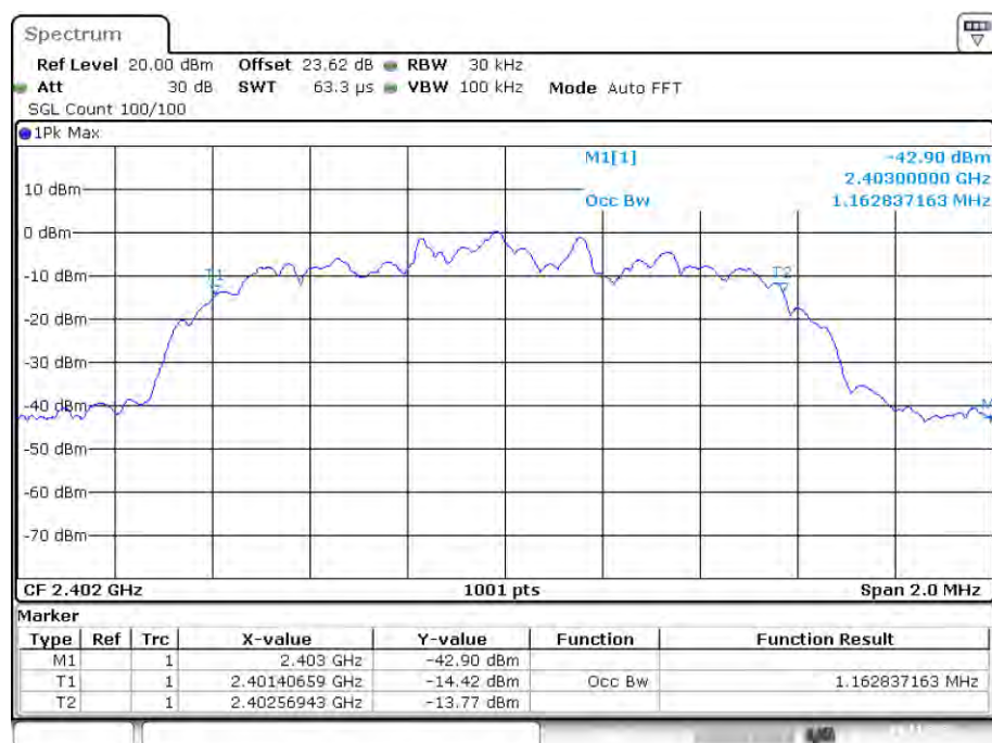
OBW NVNT 2-DH1 2402MHz Ant1
