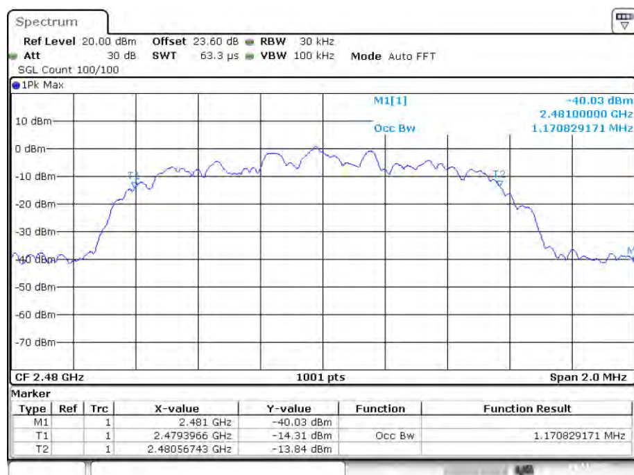
OBW NVNT 2-DH1 2480MHz Ant1
