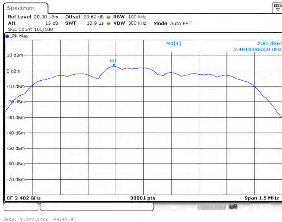
Tx. Spurious NVNT 2-DH1 2402MHz Ant1 Emission
