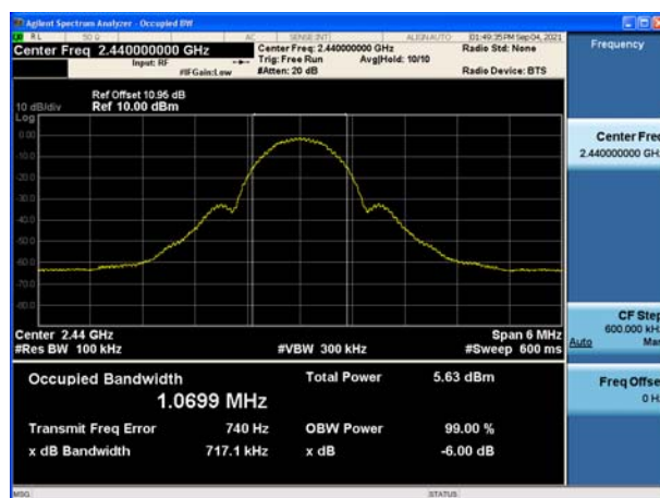
Modulation: Coded 125K 2440MHz
