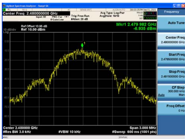
Modulation: 1Mbps 2480MHz
