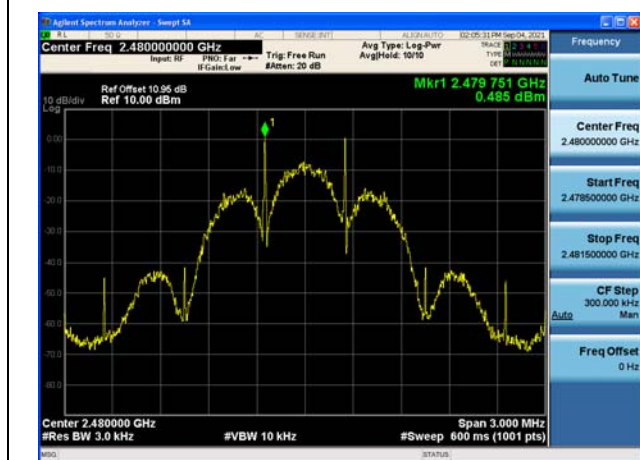
Modulation: Coded 250K 2480MHz
