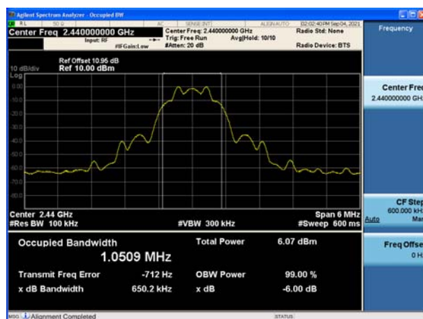
Modulation: Coded 250K 2440MHz
