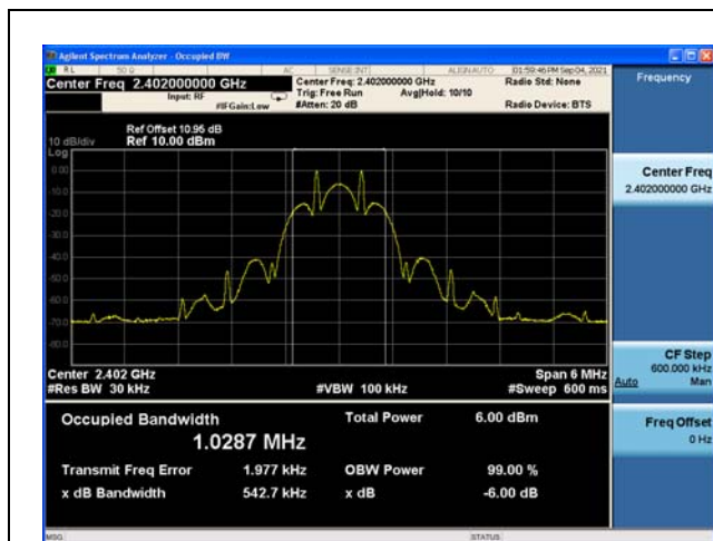
Modulation: Coded 250K 2402MHz
