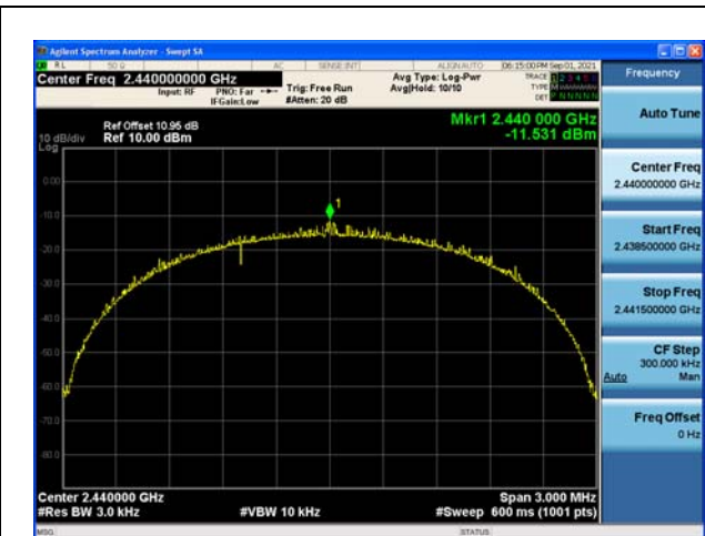
Modulation: 2Mbps 2440MHz
