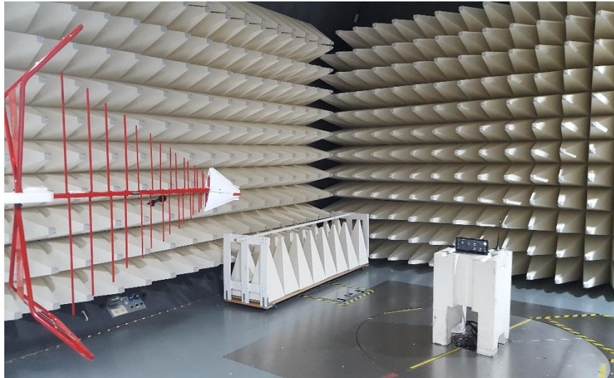
Figure B5. Radiated emission Setup 1
