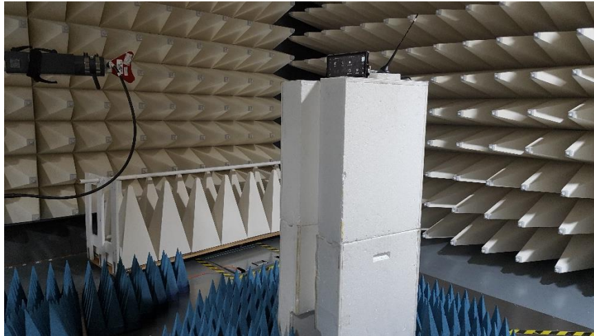
Figure B7. Radiated emission Setup 3
