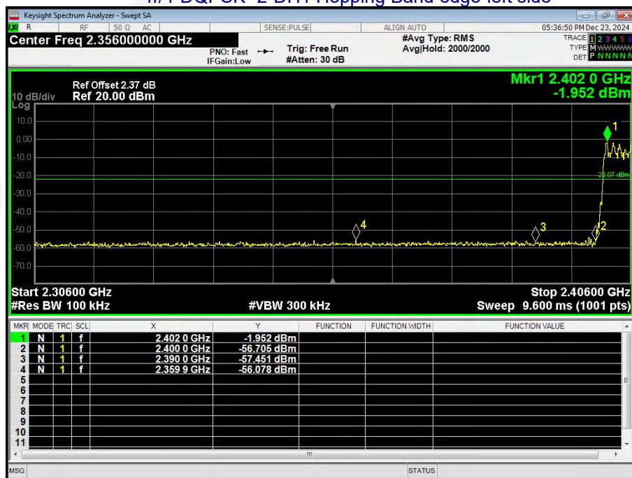
\pi/4 -DQPSK -2-DH1 Hopping Band edge-left side
