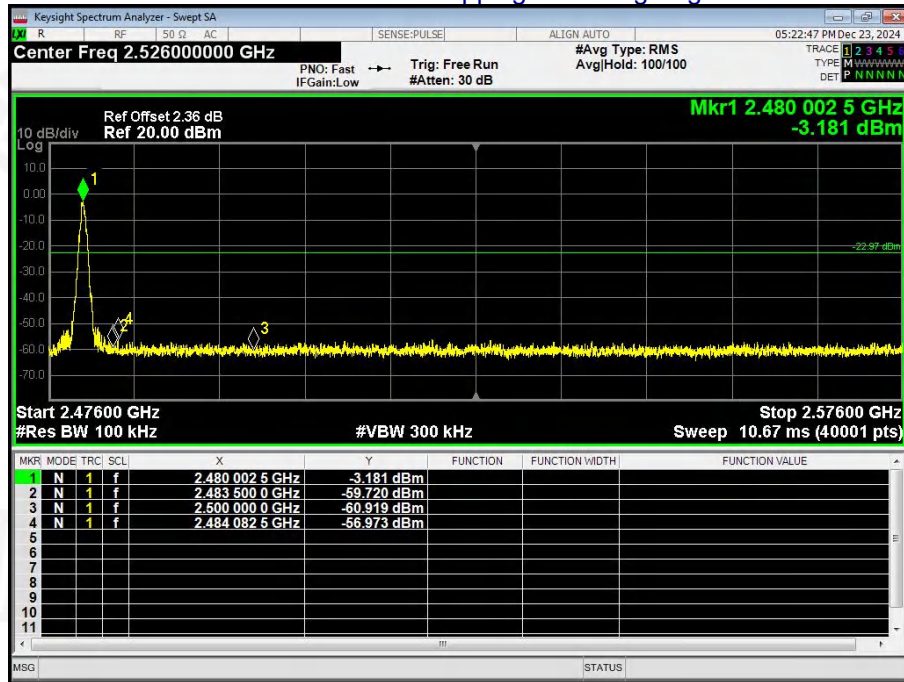
GFSK -1-DH1 No-hopping Band edge-right side
