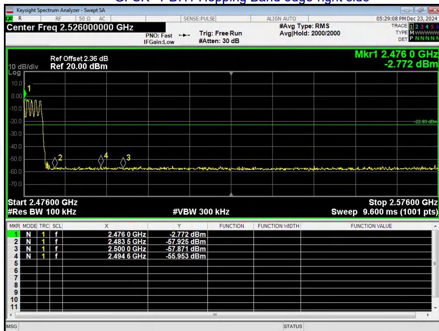
GFSK -1-DH1 Hopping Band edge-right side
