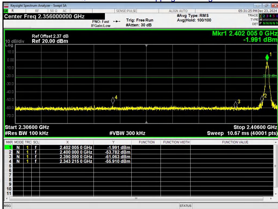
\pi/4 -DQPSK -2-DH1 No-hopping Band edge-left side
