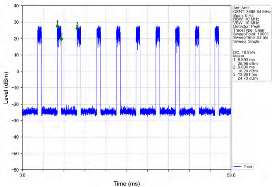
n48_30kHz_SISO_NTNV_20MHz_CP-OFDM_64_QAM_3690MHz_Inner_1RB_Right_Ant1
