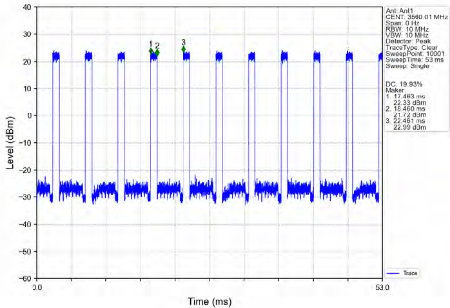
n48_30kHz_SISO_NTNV_20MHz_CP-OFDM 64 QAM_3560.01MHz_Inner_Full_Ant1
