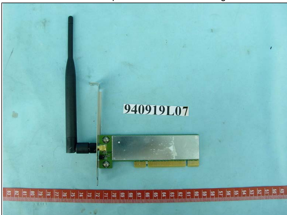
Antenna 1: Dipole antenna with 4.98dBi gain
