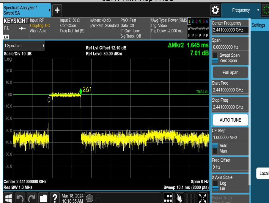
3DH3-Ant1-Hop-PASS
