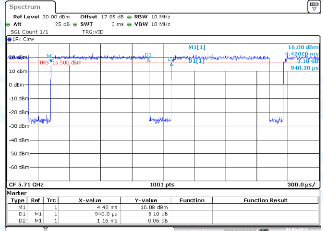
NTNV-11N40MIMO-Ant2-5710
