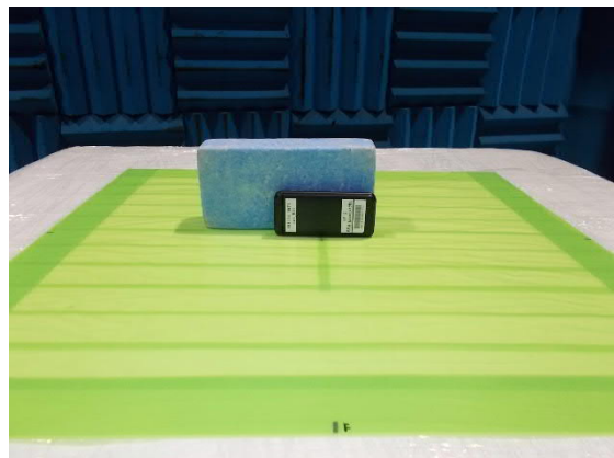
Z-axis, Close
