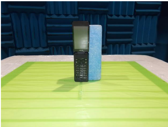
Z-axis, Open
