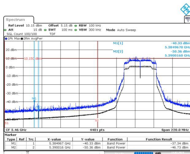
BE-R-LOW, MIMO-B, 802.11ax/be40-MCS0, Ch102
