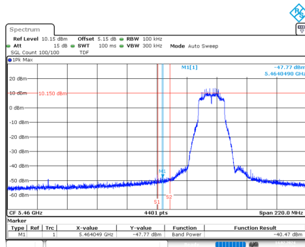
BE-NR-LOW, MIMO-B, 802.11ax/be20-MCS0, Ch100
