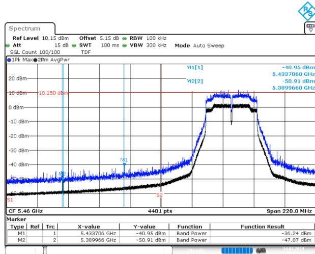
BE-R-LOW, MIMO-B, 802.11n40-HT8, Ch102
