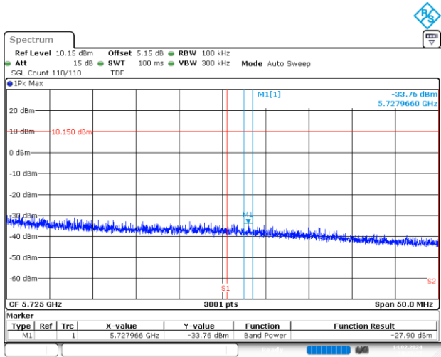
BE-NR-HIGH, SISO-B, 802.11ax/be40-MCS0, Ch134
