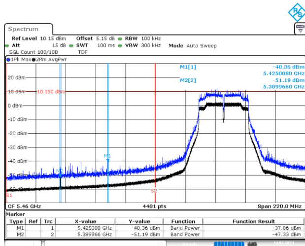
BE-R-LOW, MIMO-A, 802.11n40-HT8, Ch102
