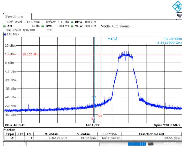
BE-NR-LOW, MIMO-B, 802.11n20-HT8, Ch100
