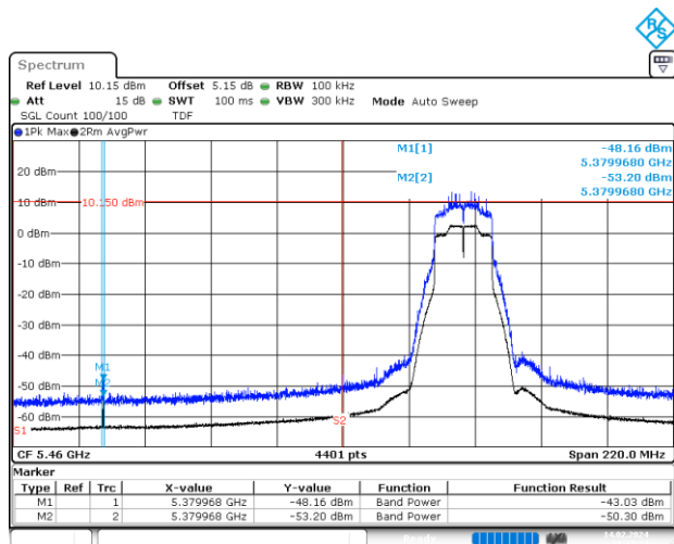
BE-R-LOW, MIMO-B, 802.11ax/be20-MCS0, Ch100
