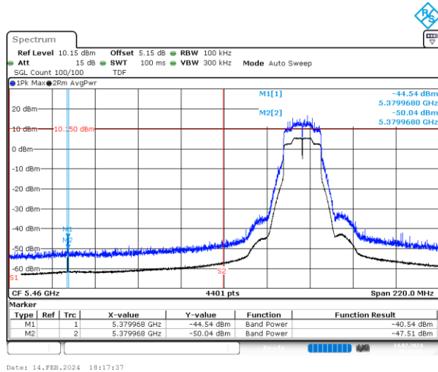
BE-R-LOW, SISO-B, 802.11ax/be20-MCS0, Ch100
