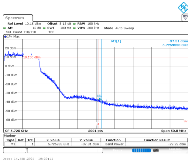
BE-NR-HIGH, SISO-B, 802.11ax/be20-MCS0, Ch140
