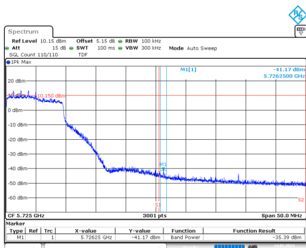
BE-NR-HIGH, MIMO-B, 802.11ax/be20-MCS0, Ch140
