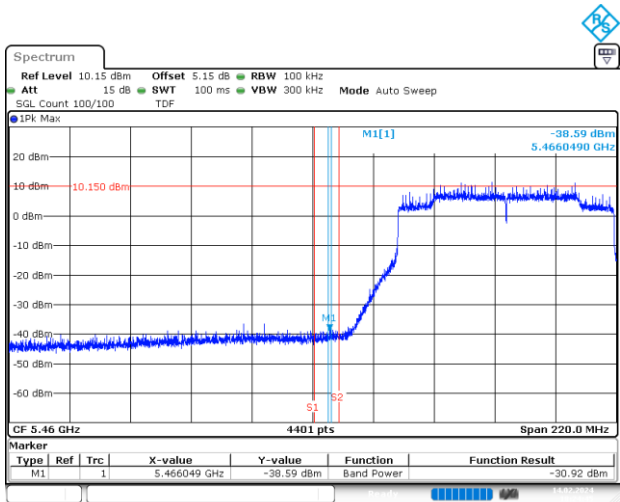
BE-NR-LOW, SISO-B, 802.11ax/be80-MCS0, Ch106
