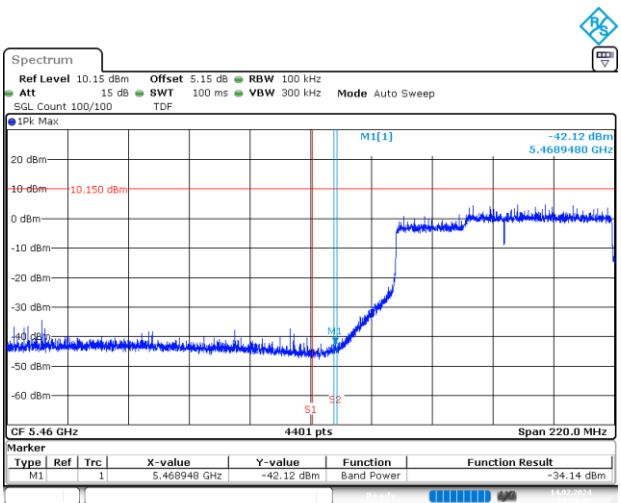
BE-NR-LOW, SISO-B, 802.11ax/be160-MCS0, Ch114
