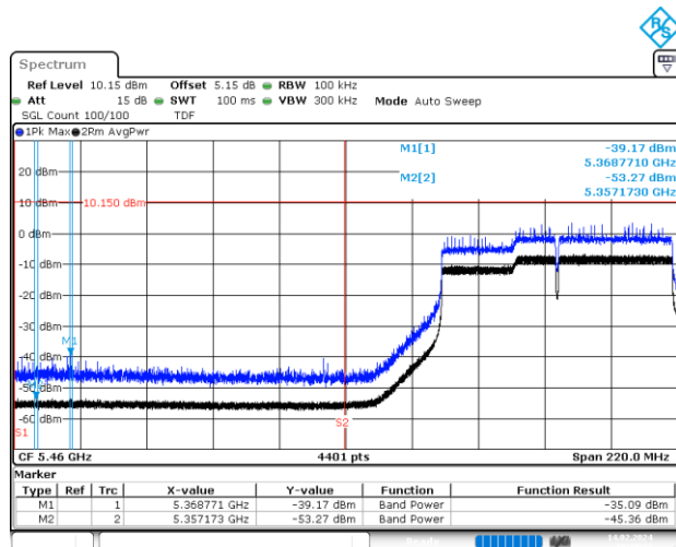
BE-NR-LOW, MIMO-A, 802.11ac160-VHT8, Ch112
