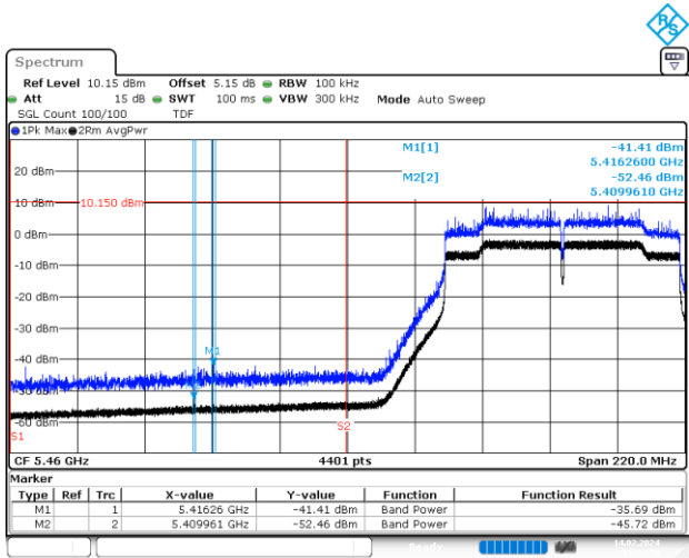
BE-R-LOW, MIMO-B, 802.11ac80-VHT8, Ch106
