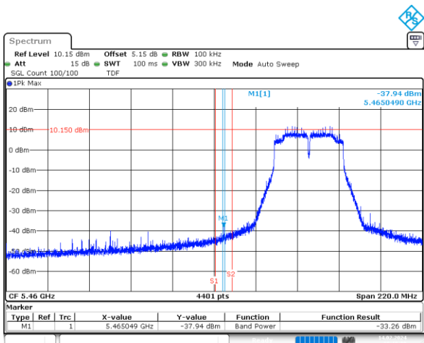
BE-NR-LOW, MIMO-A, 802.11n40-HT8, Ch102
