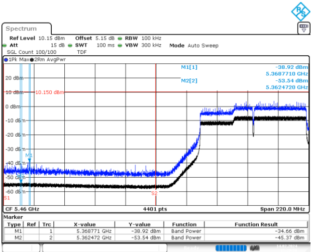
BE-R-LOW, MIMO-B, 802.11ac160-VHT8, Ch114
