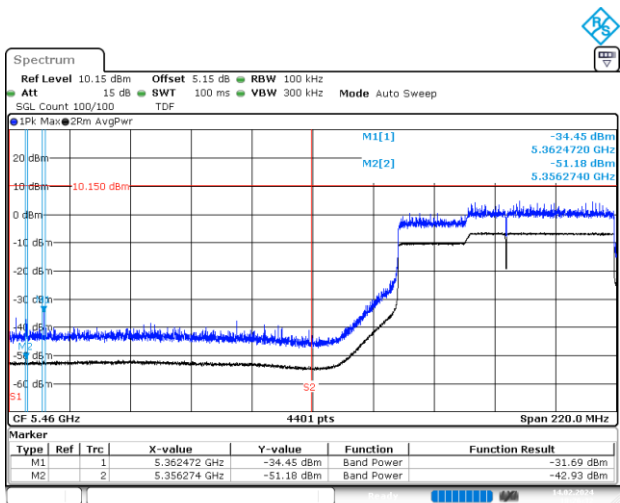
BE-R-LOW, SISO-B, 802.11ax/be160-MCS0, Ch114
