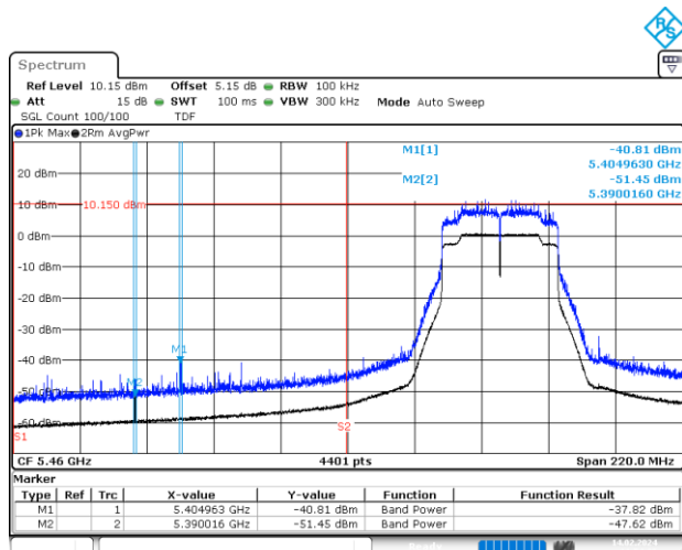
BE-R-LOW, MIMO-A, 802.11ax/be40-MCS0, Ch102
