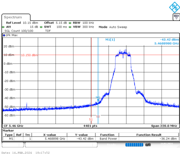
BE-NR-LOW, SISO-B, 802.11ax/be20-MCS0, Ch100
