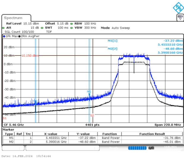
BE-R-LOW, SISO-B, 802.11ax/be40-MCS0, Ch102
