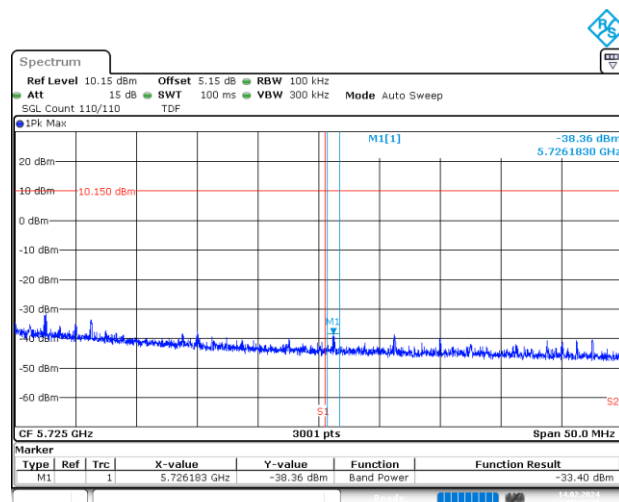
BE-NR-HIGH, MIMO-B, 802.11ax/be40-MCS0, Ch134
