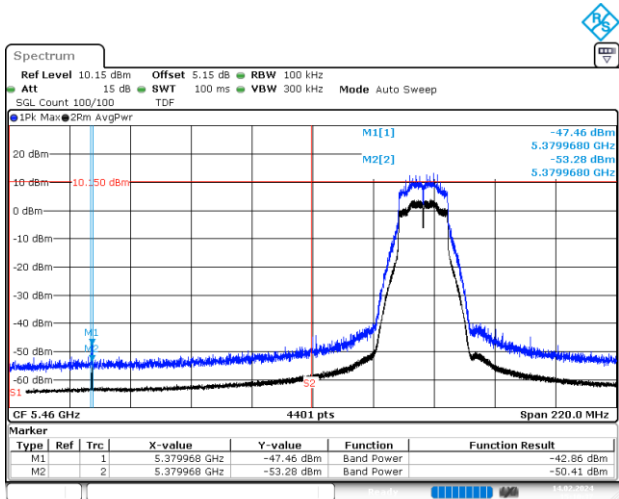
BE-R-LOW, MIMO-B, 802.11n20-HT8, Ch100
