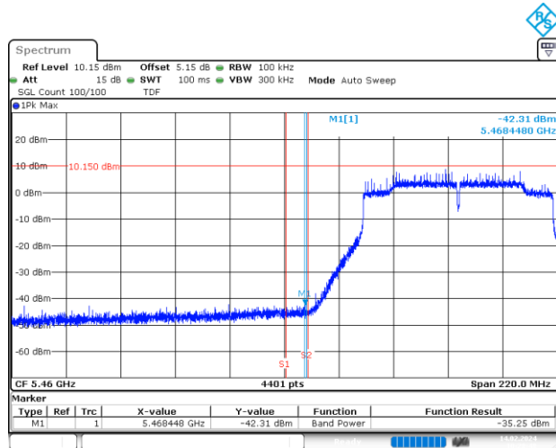
BE-NR-LOW, MIMO-A, 802.11ac80-VHT8, Ch106
