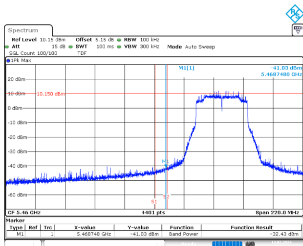
BE-NR-LOW, MIMO-B, 802.11ax/be40-MCS0, Ch102
