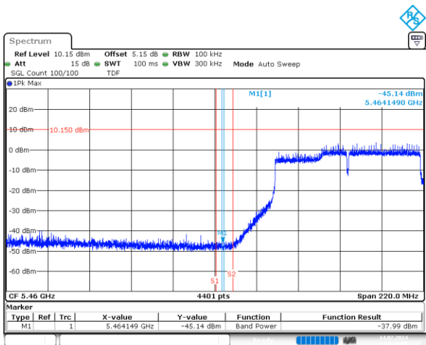
BE-NR-LOW, MIMO-B, 802.11ac160-VHT8, Ch114
