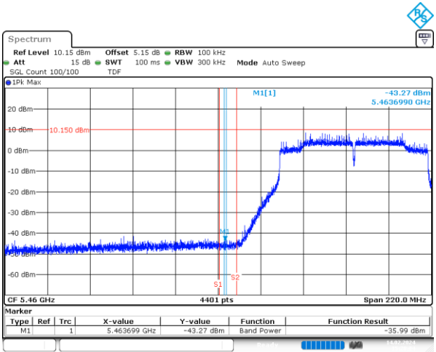
BE-NR-LOW, MIMO-B, 802.11ac80-VHT8, Ch106
