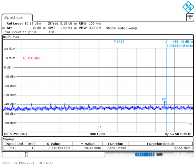
BE-NR-HIGH, SISO-B, 802.11ac160-VHT0, Ch114
