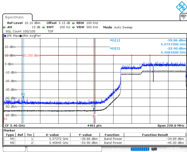
BE-R-LOW, MIMO-A, 802.11ax/be160-MCS0, Ch114
