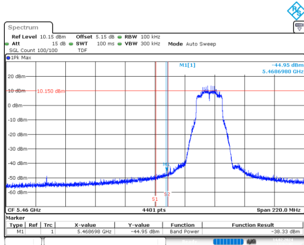
BE-NR-LOW, MIMO-A, 802.11ax/be20-MCS0, Ch100
