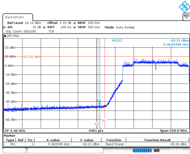
BE-NR-LOW, MIMO-A, 802.11ax/be80-MCS0, Ch106
