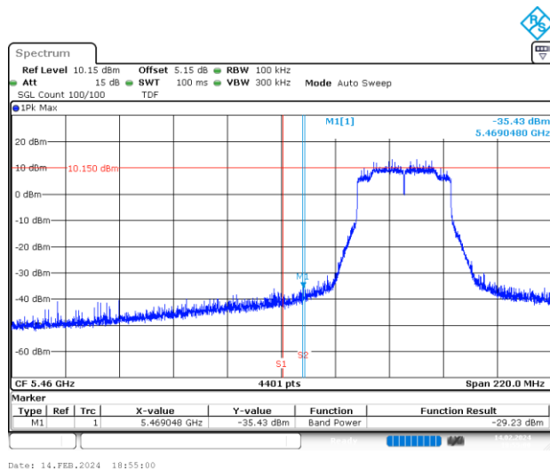
BE-NR-LOW, SISO-B, 802.11ax/be40-MCS0, Ch102
