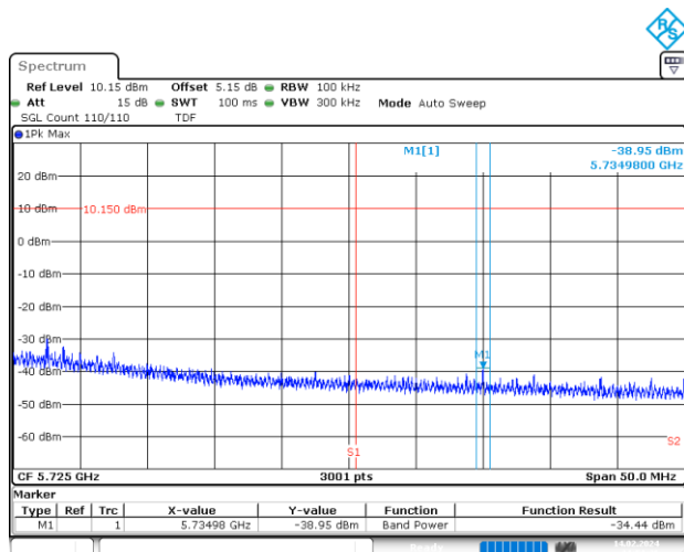
BE-NR-HIGH, MIMO-A, 802.11n40-HT8, Ch134
