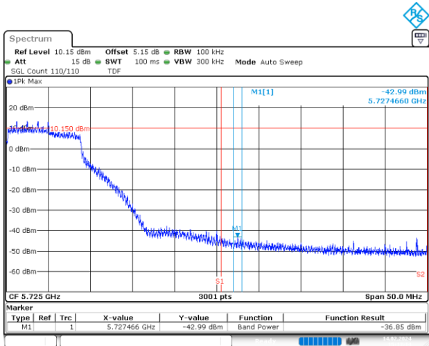
BE-NR-HIGH, MIMO-B, 802.11n20-HT8, Ch140
