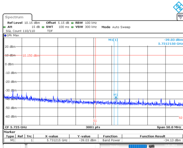
BE-NR-HIGH, MIMO-B, 802.11n40-HT8, Ch132
