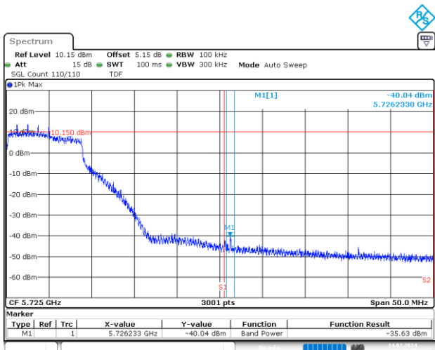
BE-NR-HIGH, MIMO-A, 802.11n20-HT8, Ch140
