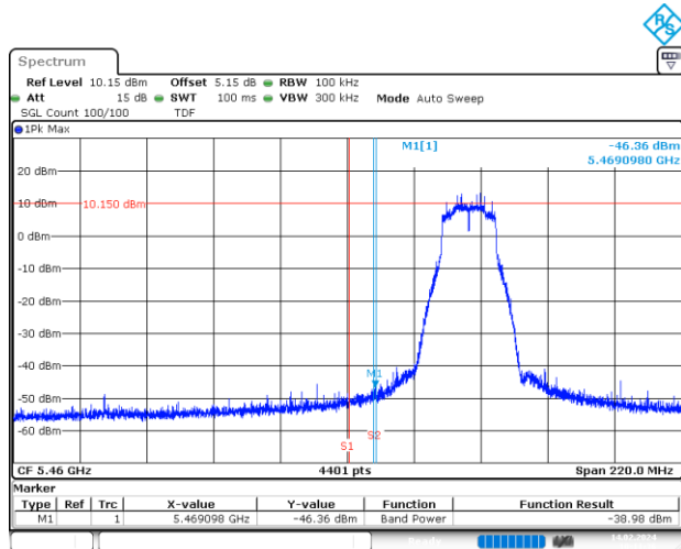
BE-R-LOW, MIMO-A, 802.11n20-HT8, Ch100
