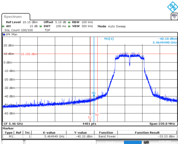
BE-NR-LOW, MIMO-B, 802.11n40-HT8, Ch102
