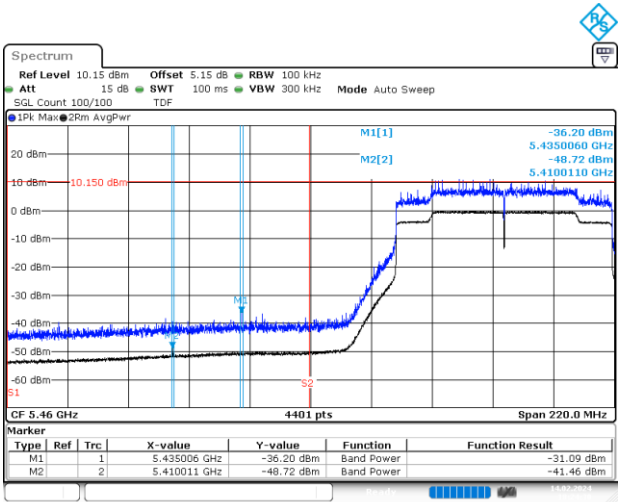
BE-R-LOW, SISO-B, 802.11ax/be80-MCS0, Ch106
