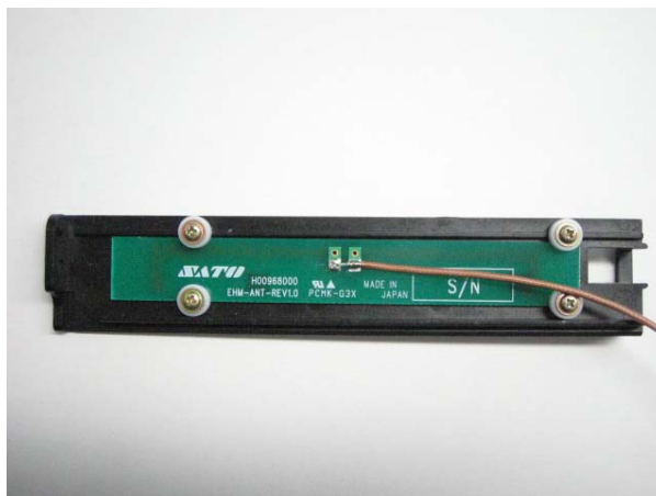
Antenna Holder
