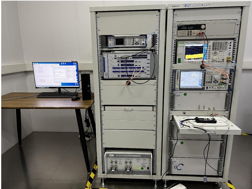
Conducted Test For WWAN
