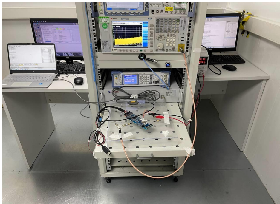
Conducted Test for BLE
