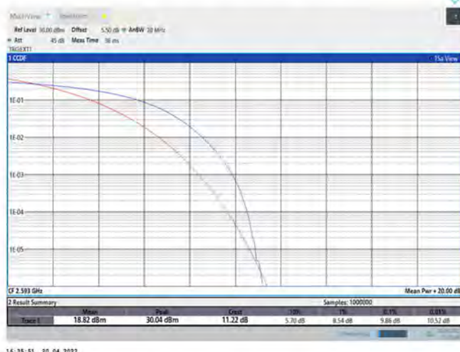
41-41-20MHz-20MHz-QPSK-QPSK-40521-40719-100RB#0-100RB#0
