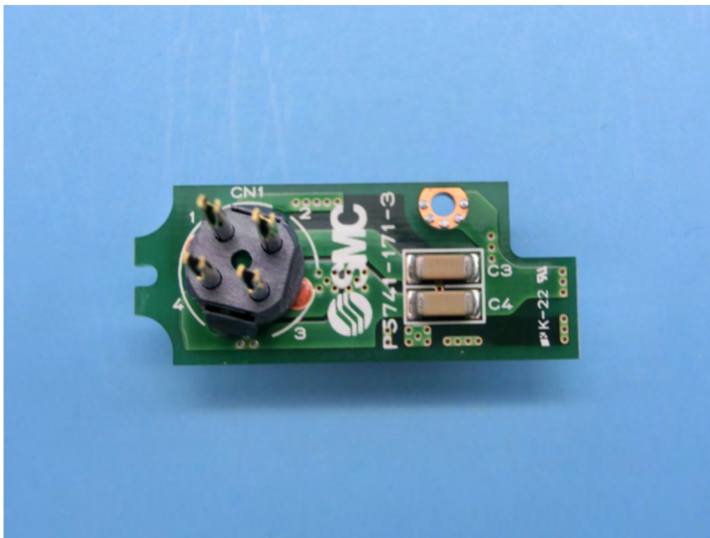
M12-4 pin connector board assembly
