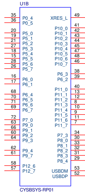
Figure 7. Castellated Pads Pinout
