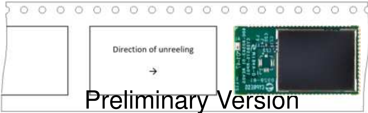
Figure 9. Tape Dimensions
