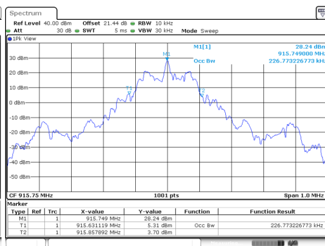
99% Occupied Bandwidth Plot on 915.75 MHz
