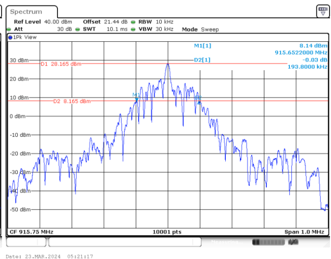
20 dB Bandwidth Plot on 915.75 MHz
