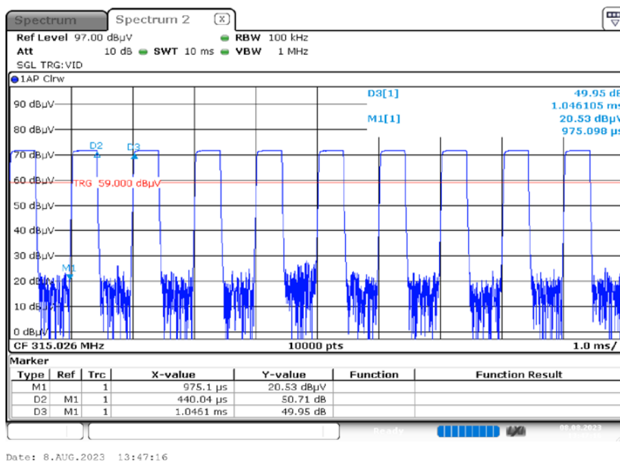
Plot 2: Timing of the transmitter
