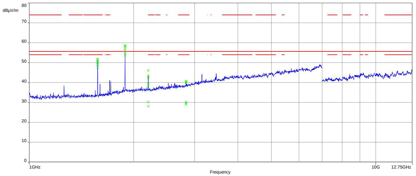
Plot 3: 1000 MHz to 12.75 GHz, vertical & horizontal polarisation
