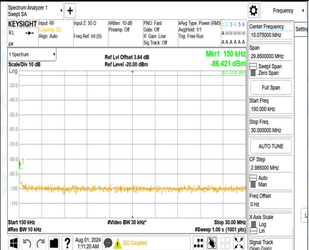
Band5_3MHz_16QAM_20525_1RB#0_1000~3000_1000~3000
