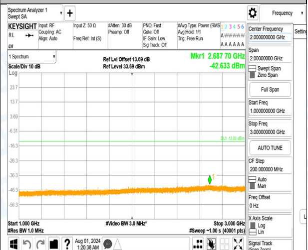
Band5_3MHz_16QAM_20635_1RB#14_1000~3000_1000~3000
