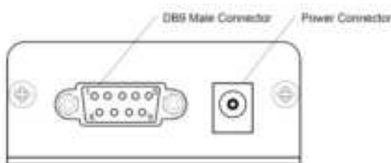
Figure 1: CL4490-RS232
