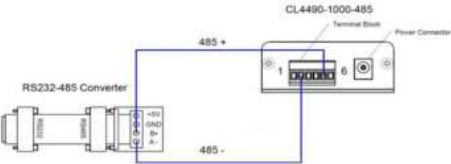
Figure 5: RS232-485 Converter
