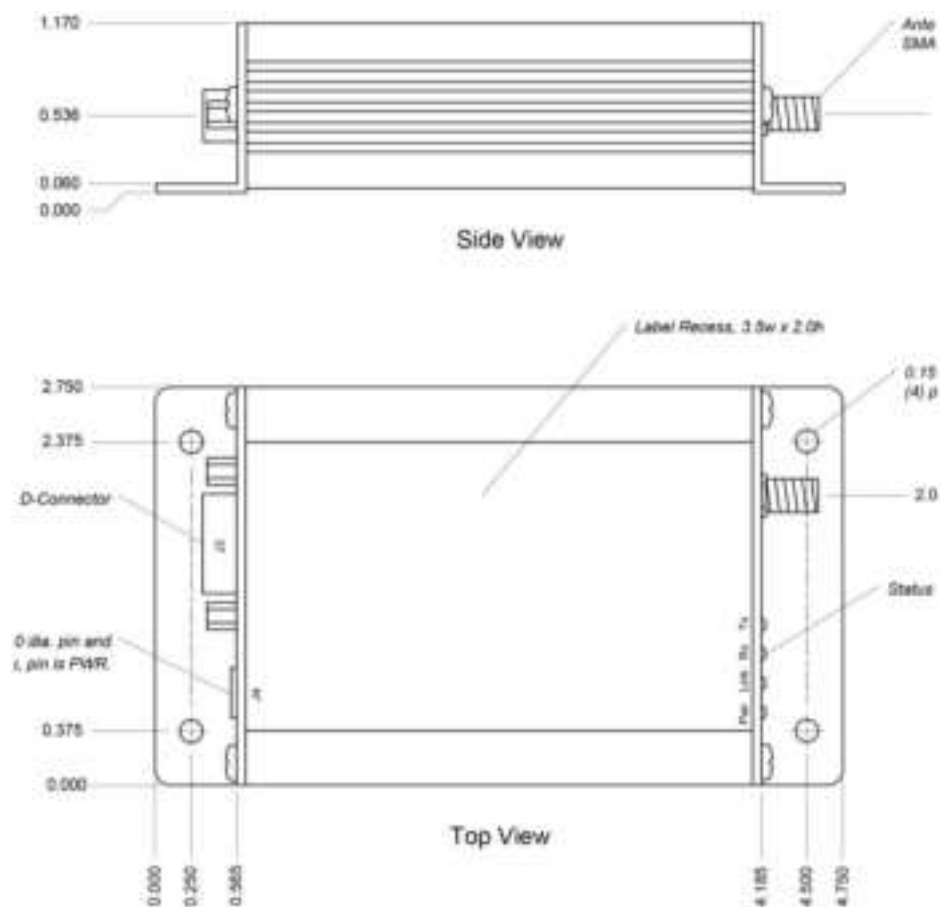
Figure 11: CL4490 Mechanical
