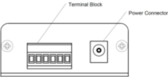
Figure 4: CL4490-RS485
