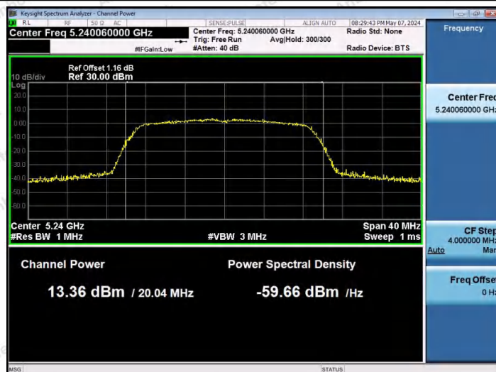
11AC20SISO-Ant1-5240-PASS
