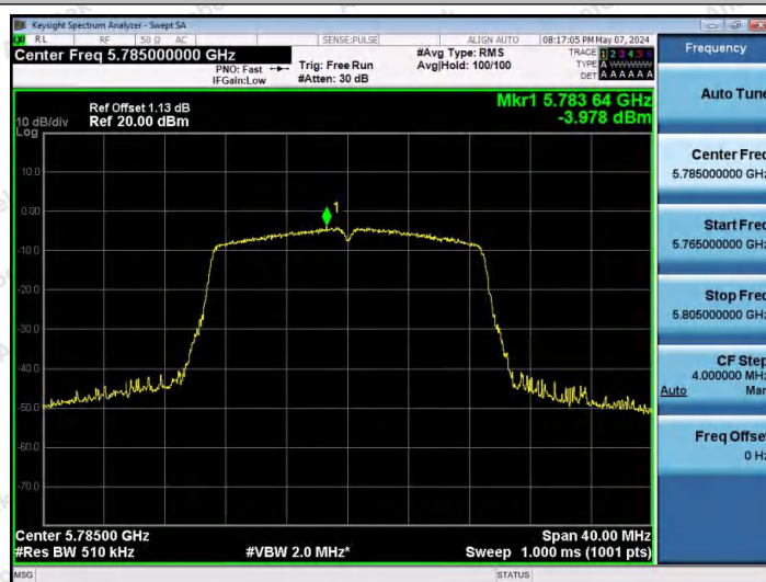
11N20SISO-Ant1-5785-PASS
