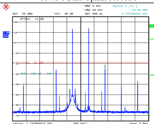
AWS-1 Band Uplink-Pre AGC
