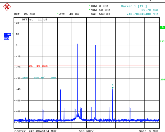
Lower 700MHz Band Downlink -Max. Input Level
