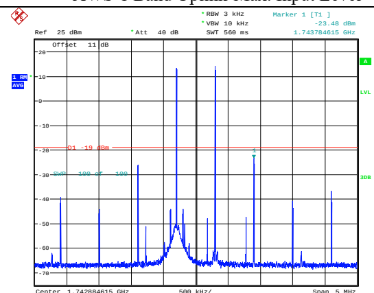
AWS-1 Band Uplink-Max. Input Level
