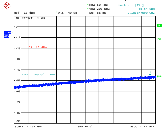
Left Side-WCDMA-Max. Input Level
