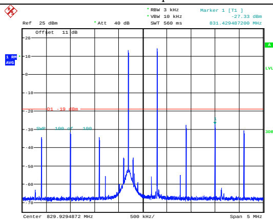
Cellular Band Uplink-Pre AGC
