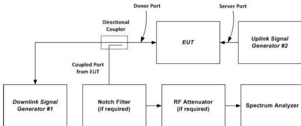
Figure 5 – Variable gain instrumentation test setup
