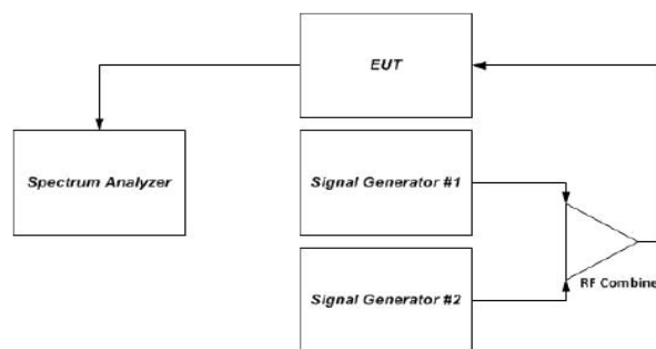
Figure 2 – Intermodulation product instrumentation test setup
