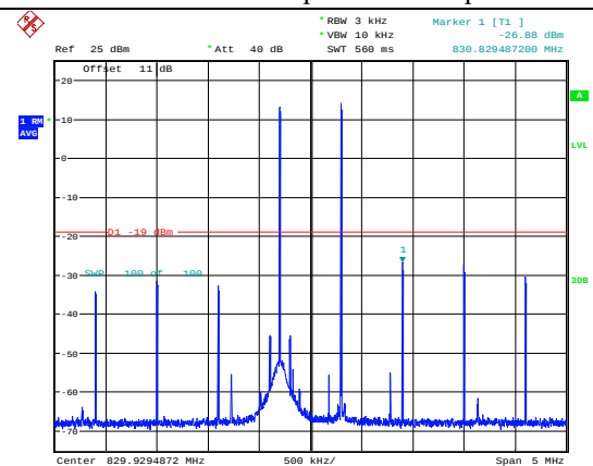
Cellular Band Uplink-Max. Input Level
