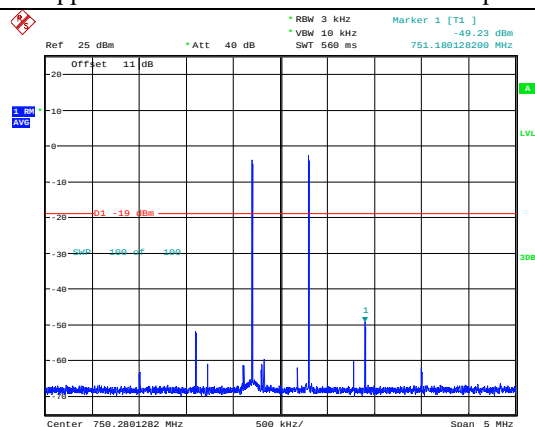
Upper 700MHz Band Downlink -Max. Input Level
