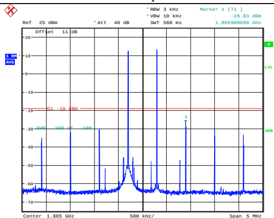
PCS Band Uplink-Pre AGC
