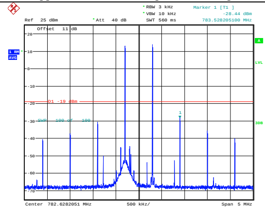
Upper 700MHz Band Uplink-Max. Input Level
