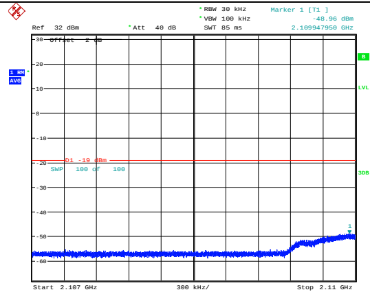
Left Side-CDMA-Max. Input Level
