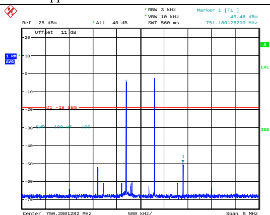
Upper 700MHz Band Downlink -Pre AGC
