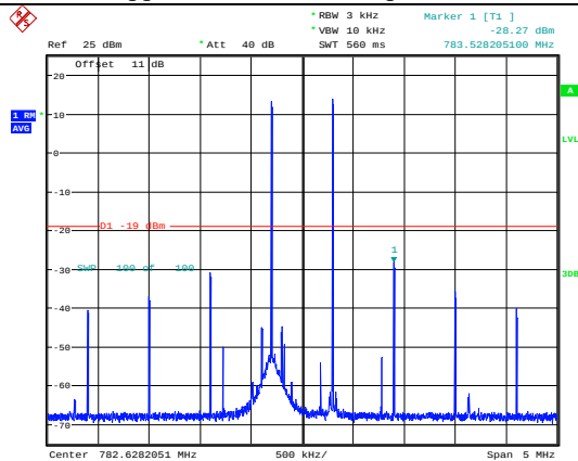
Upper 700MHz Band Uplink-Pre AGC
