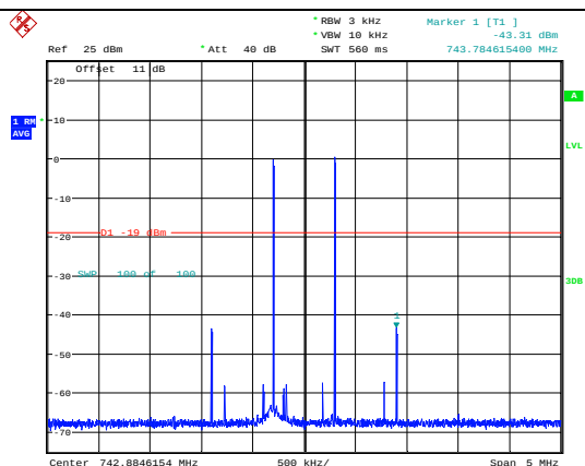
Lower 700MHz Band Downlink-Pre AGC
