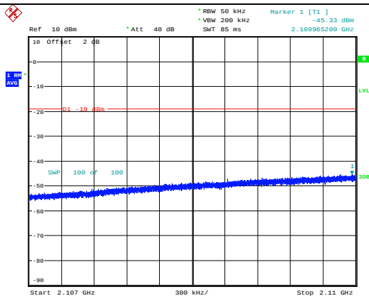
Left Side-WCDMA-Pre AGC
