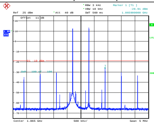
PCS Band Uplink-Max. Input Level
