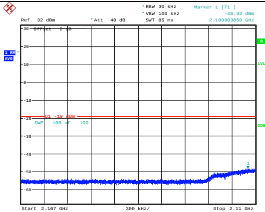
Left Side-CDMA-Pre AGC
