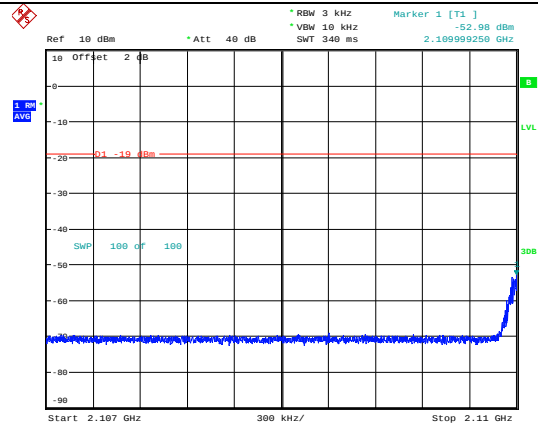
Left Side-GSM-Max. Input Level
