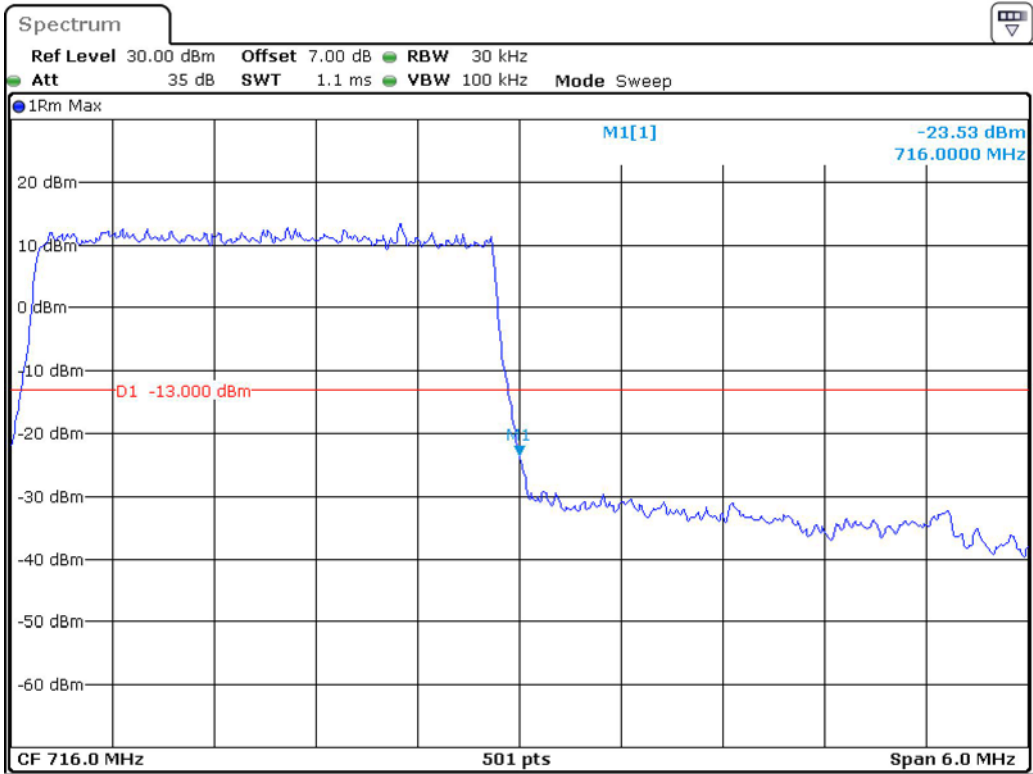
Band 12_3 MHz_High_QPSK_RB15#0
