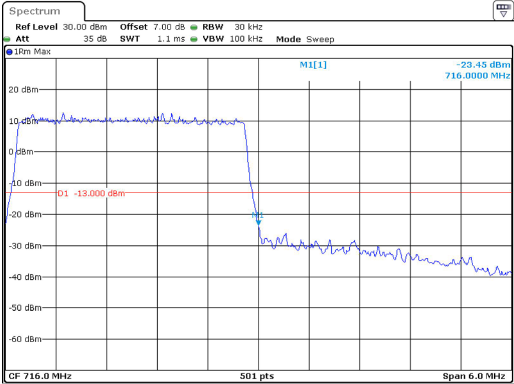
Band 12_3 MHz_High_16QAM_RB15#0
