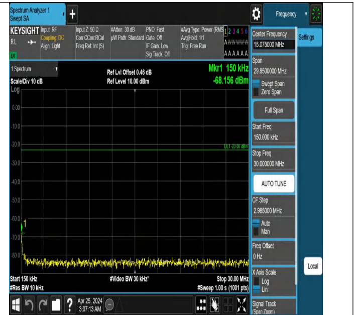
Band12_5MHz_QPSK_23035_1RB#0_0.15~30_0.15~30
