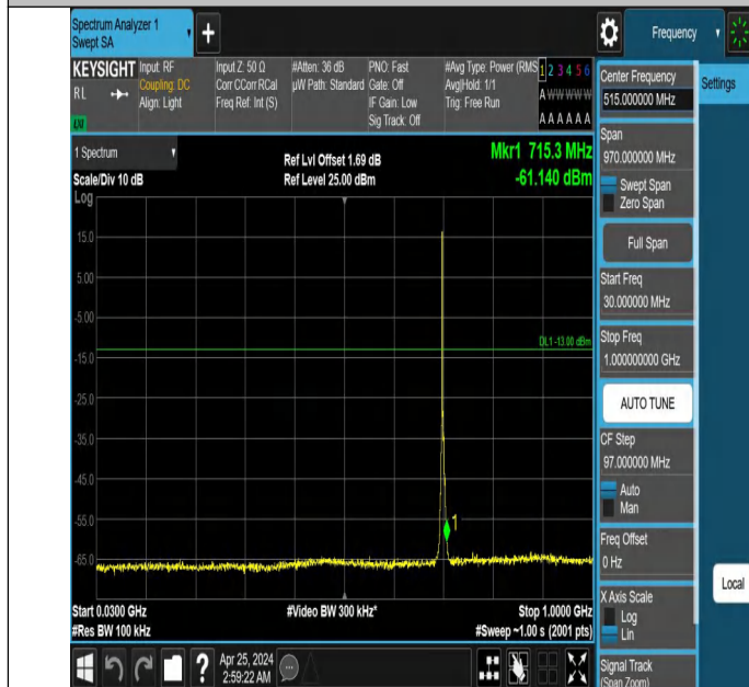
Band12_3MHz_QPSK_23095_1RB#0_30~1000_30~1000
