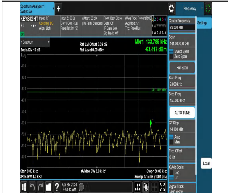
Band12_3MHz_QPSK_23025_1RB#0_0.009~0.15_0.009~0.15
