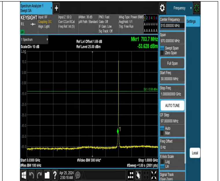
Band12_1.4MHz_QPSK_23095_1RB#5_30~1000_30~1000
