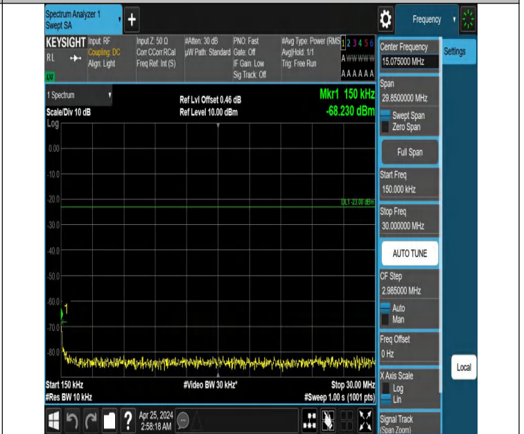
Band12_3MHz_QPSK_23025_1RB#0_0.15~30_0.15~30
