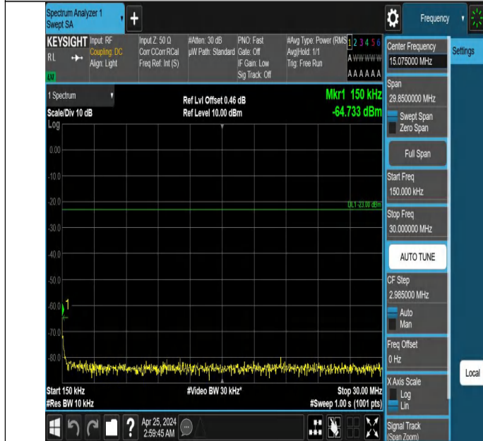
Band12_3MHz_QPSK_23095_1RB#14_0.15~30_0.15~30
