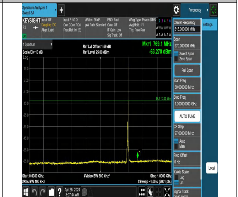
Band12_5MHz_QPSK_23035_1RB#24_30~1000_30~1000
