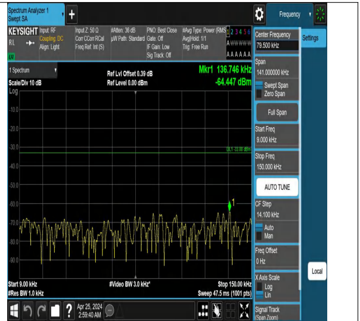
Band12_3MHz_QPSK_23095_1RB#14_0.009~0.15_0.009~0.15
