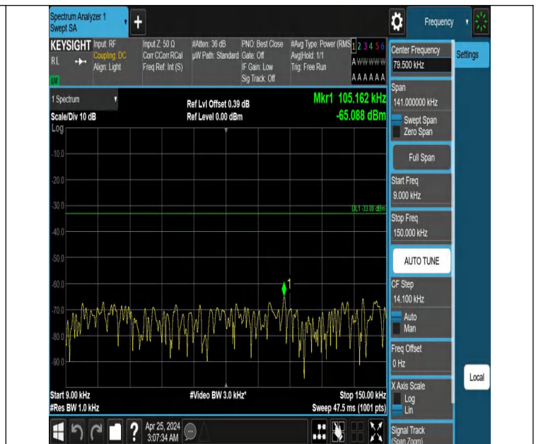
Band12_5MHz_QPSK_23035_1RB#24_0.009~0.15_0.009~0.15
