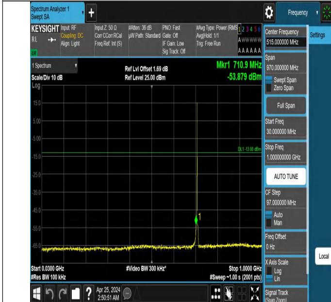
Band12_1.4MHz_QPSK_23173_1RB#0_30~1000_30~1000
