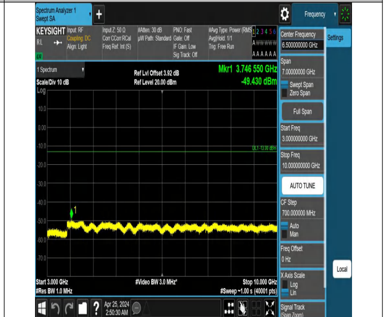
Band12_1.4MHz_QPSK_23095_1RB#5_3000~10000_3000~1000
