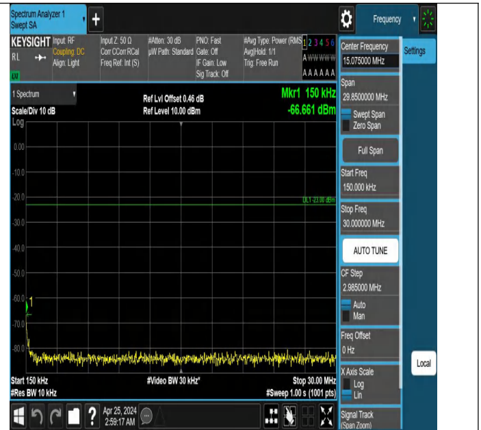
Band12_3MHz_QPSK_23095_1RB#0_0.15~30_0.15~30
