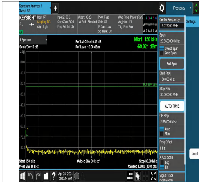
Band12_3MHz_QPSK_23165_1RB#14_0.15~30_0.15~30
