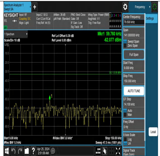
Band12_1.4MHz_QPSK_23173_1RB#5_0.009~0.15_0.009~0.15
