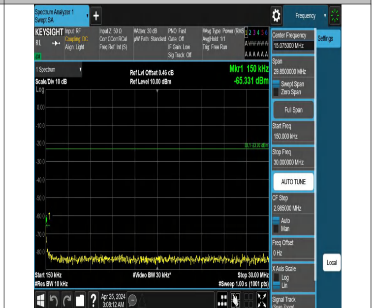
Band12_5MHz_QPSK_23095_1RB#0_0.15~30_0.15~30
