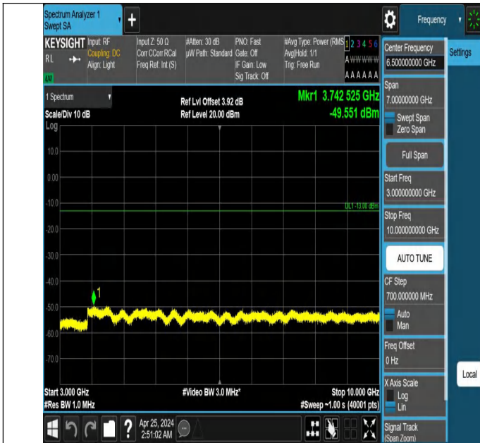
Band12_1.4MHz_QPSK_23173_1RB#0_3000~10000_3000~1000
