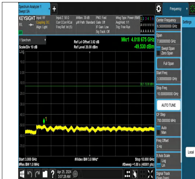
Band12_5MHz_QPSK_23035_1RB#0_3000~10000_3000~10000
