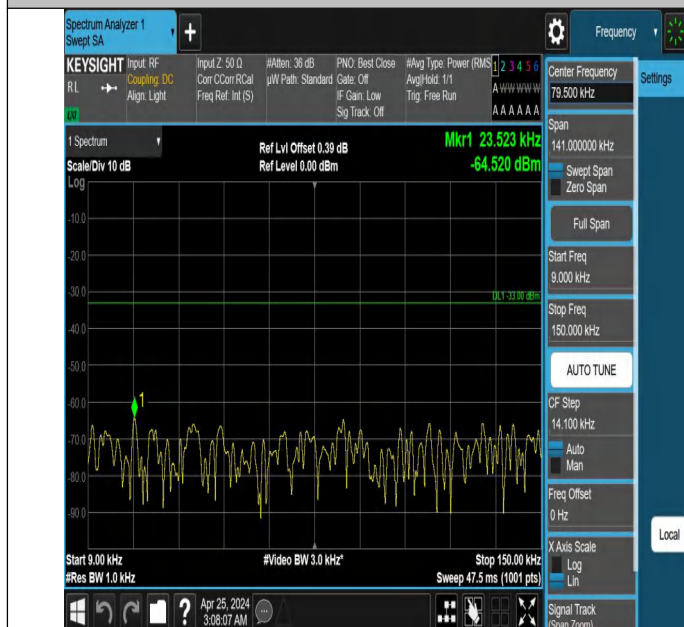
Band12_5MHz_QPSK_23095_1RB#0_0.009~0.15_0.009~0.15
