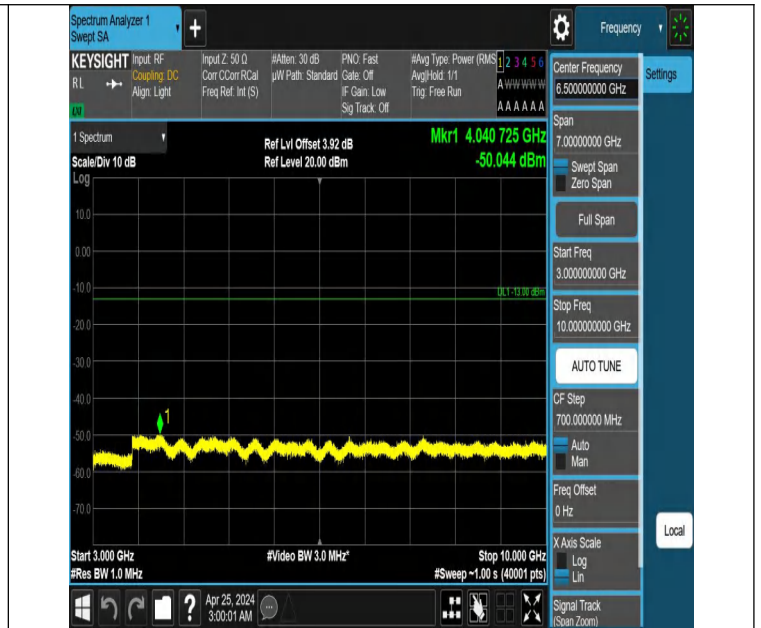
Band12_3MHz_QPSK_23095_1RB#14_3000~10000_3000~10000
