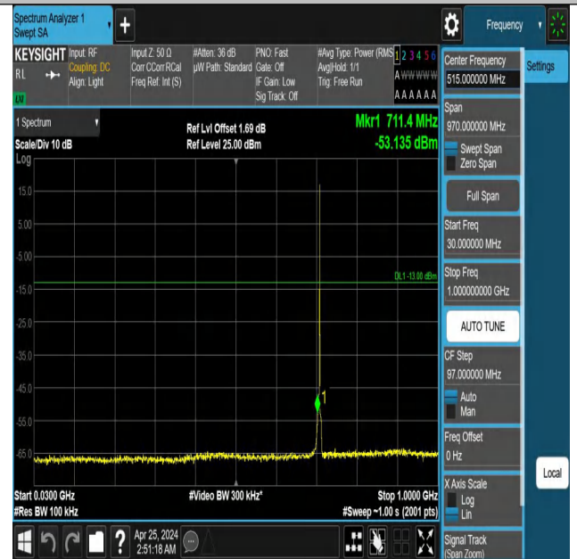
Band12_1.4MHz_QPSK_23173_1RB#5_30~1000_30~1000
