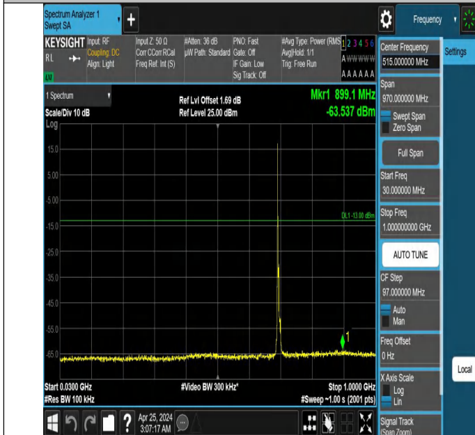
Band12_5MHz_QPSK_23035_1RB#0_30~1000_30~1000
