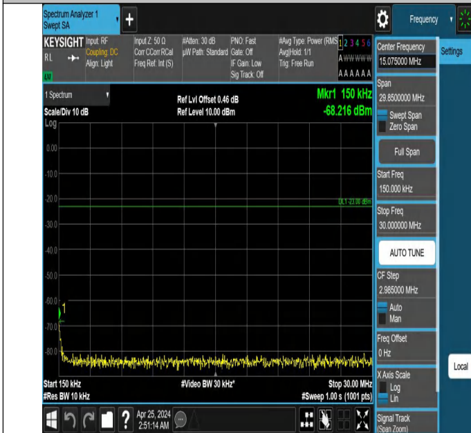
Band12_1.4MHz_QPSK_23173_1RB#5_0.15~30_0.15~30
