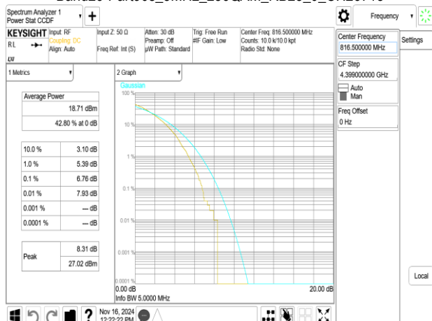
Band26-Part90s_5MHz_256QAM_RB25_0_CH26715
