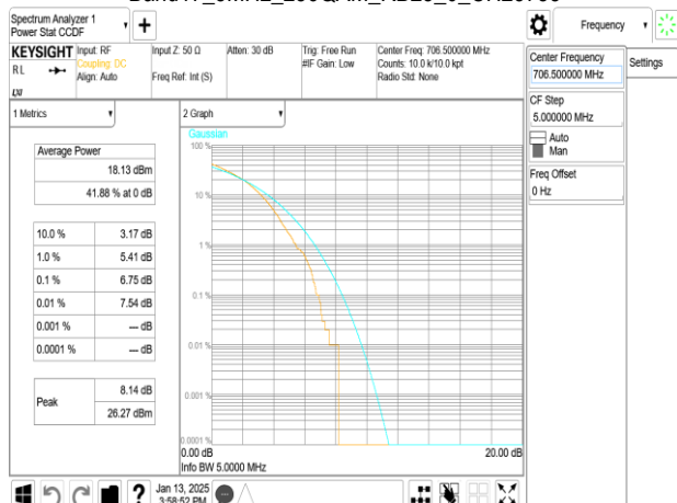
Band17_5MHz_256QAM_RB25_0_CH23755
