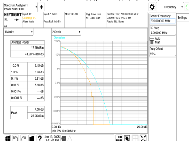
Band17_10MHz_256QAM_RB50_0_CH23780
