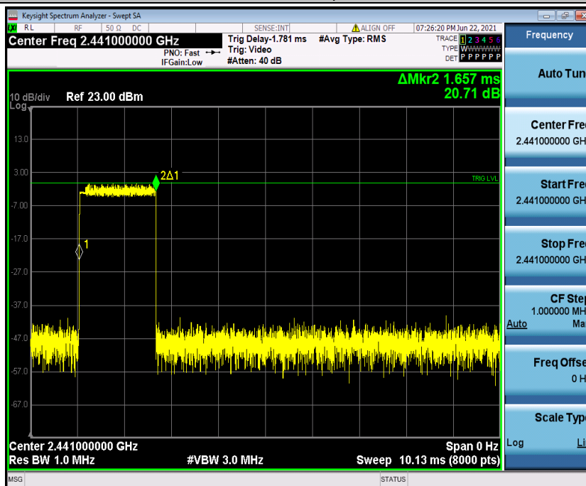
3DH3_Ant1_Hop_2441
