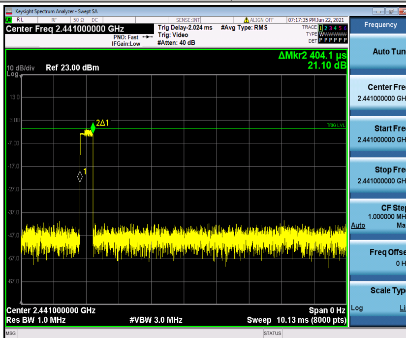
2DH1_Ant1_Hop_2441
