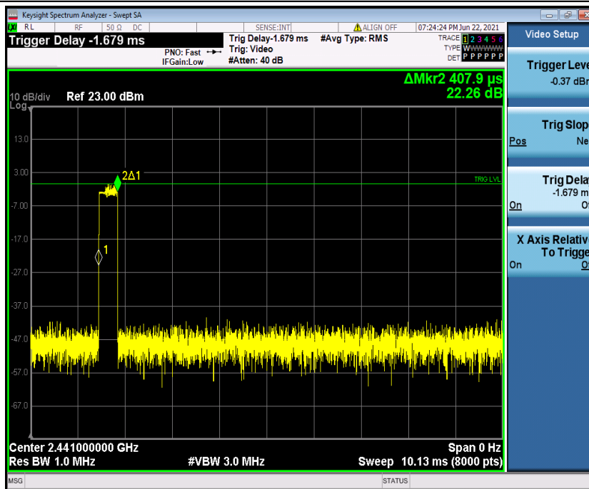
3DH1_Ant1_Hop_2441
