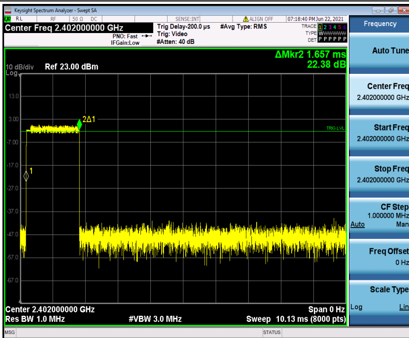
2DH3_Ant1_Hop_2402
