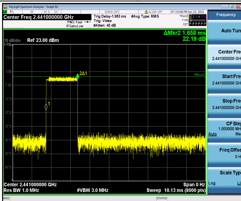
2DH3_Ant1_Hop_2441
