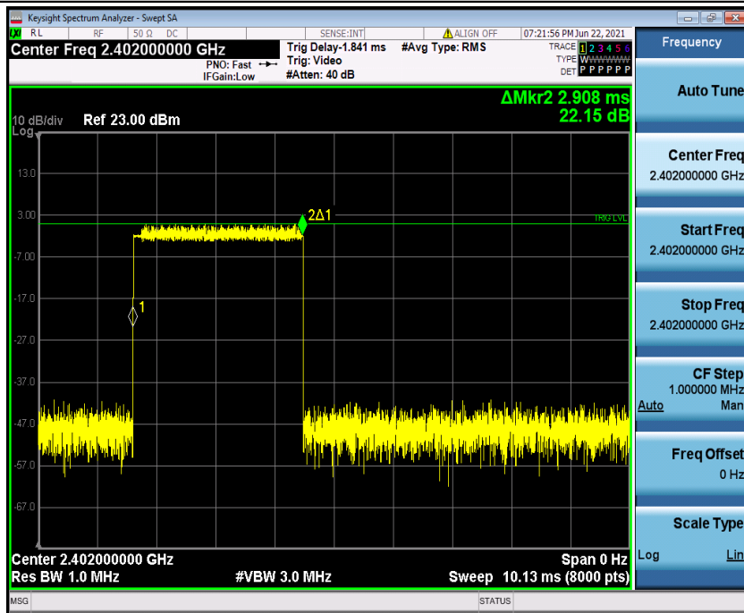
3DH5_Ant1_Hop_2402
