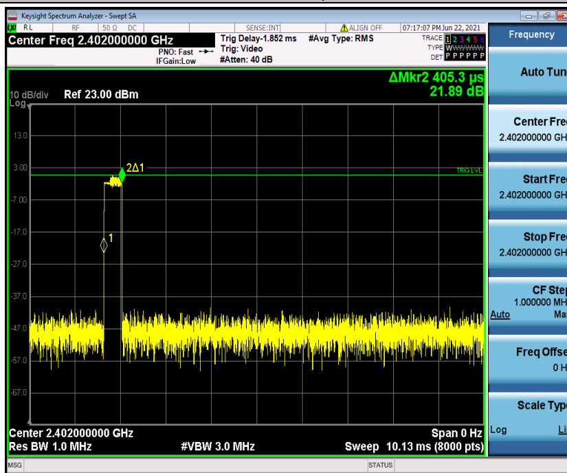
2DH1_Ant1_Hop_2402
