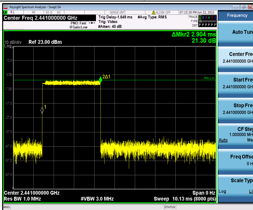
2DH5_Ant1_Hop_2441
