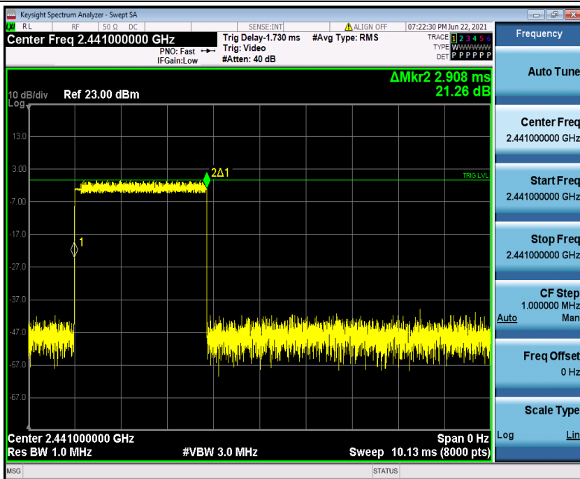
3DH5_Ant1_Hop_2441
