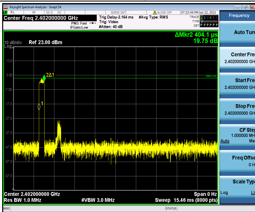
3DH1_Ant1_Hop_2402
