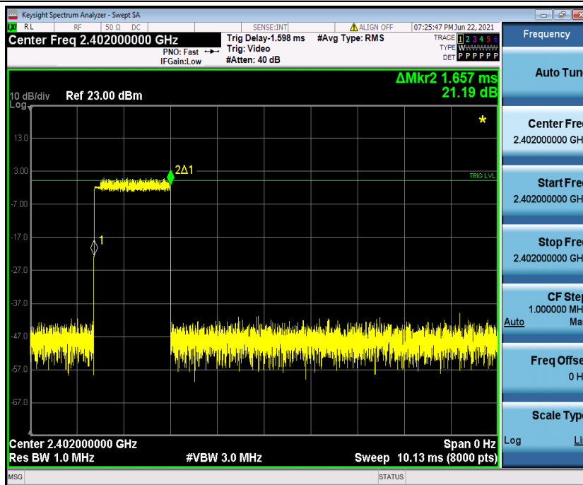
3DH3_Ant1_Hop_2402
