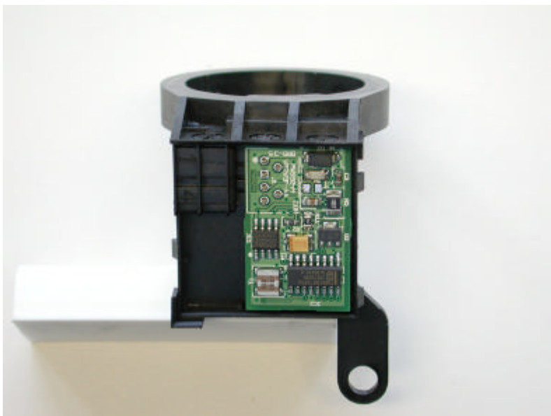
Ford 98BP Case Open
