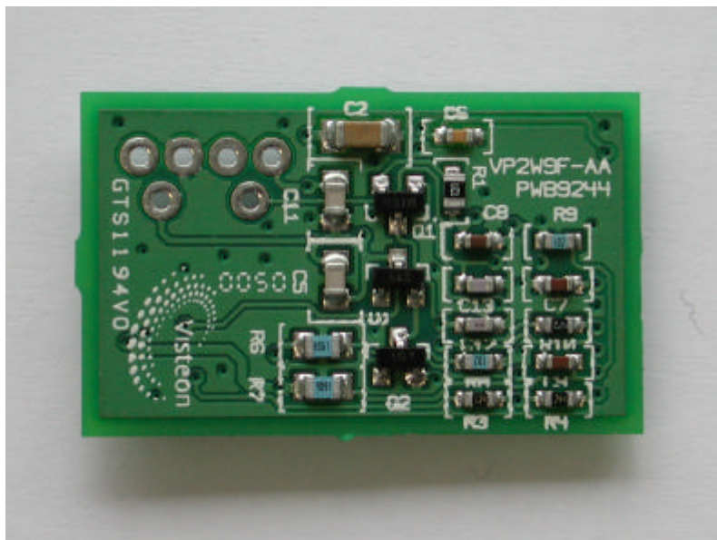
Ford 98XX PCB (top)
