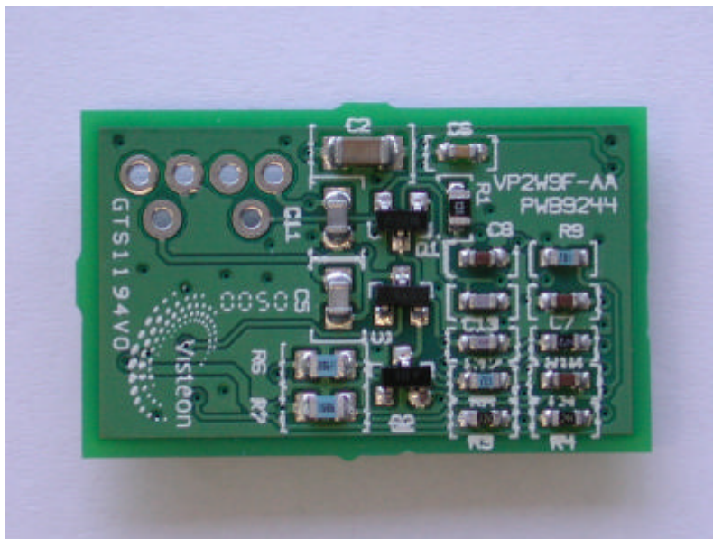
Jaguar X202/X350 PCB (bottom)
