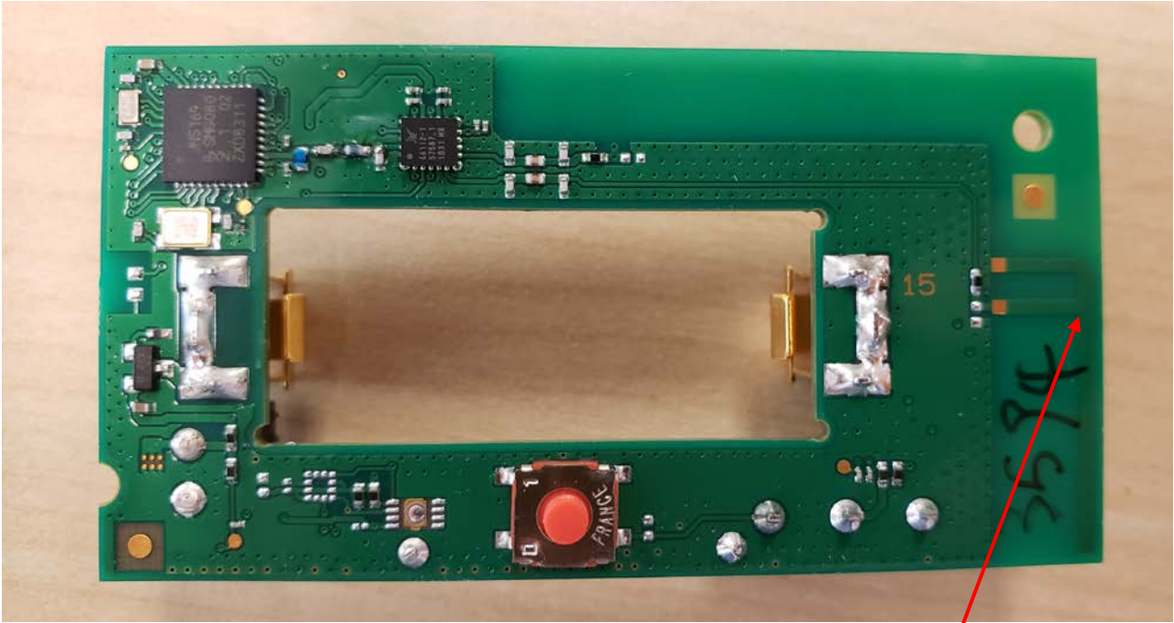
PCB BOTTOM VIEW
