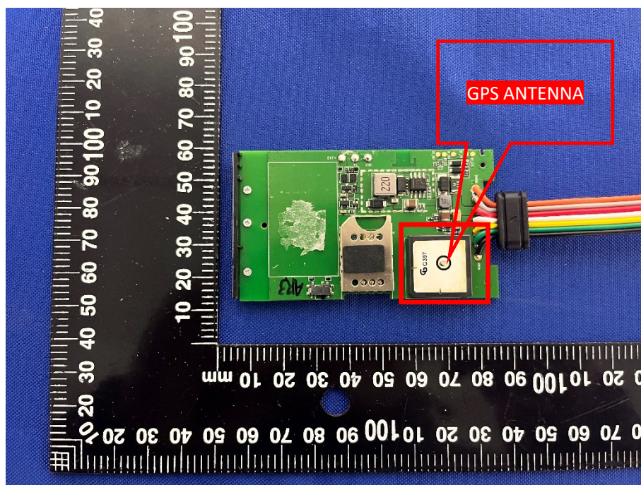
TOP VIEW OF MAINBOARD (WITHOUT SHIELD COVER)
