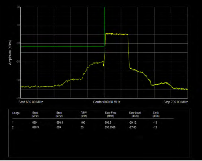
Band12 QPSK BW=3MHz Channel=23025 RB Size=1 Position=#0 Extended
