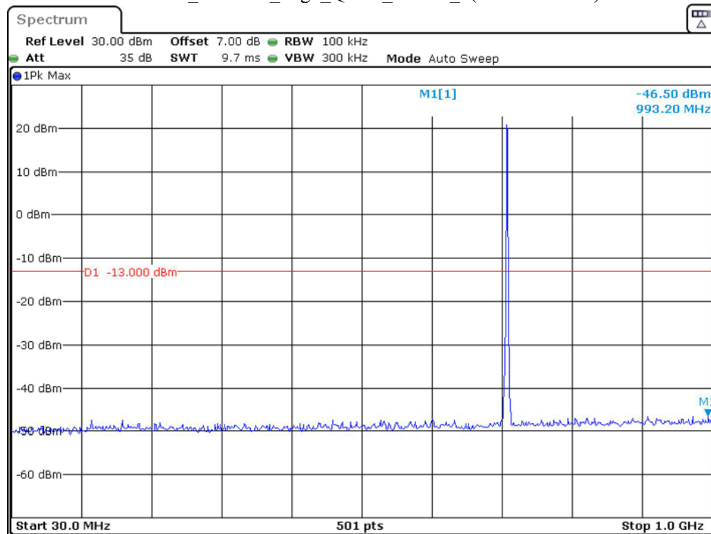
Band 12_1.4 MHz_High_QPSK_RB6#0_1(30MHz-1GHz)
