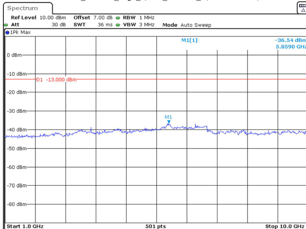
Band 12_10 MHz_High_QPSK_RB50#0_2(1GHz-10GHz)
