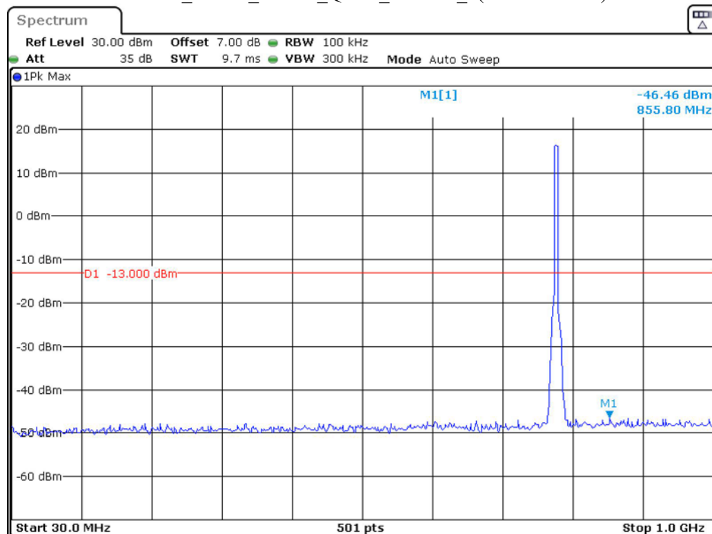
Band 13_5 MHz_Middle_QPSK_RB25#0_1(30MHz-1GHz)
