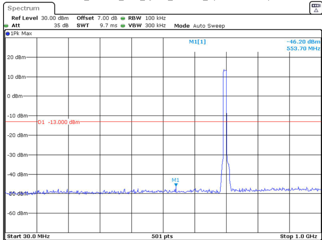
Band 12_10 MHz_Low_QPSK_RB50#0_1(30MHz-1GHz)
