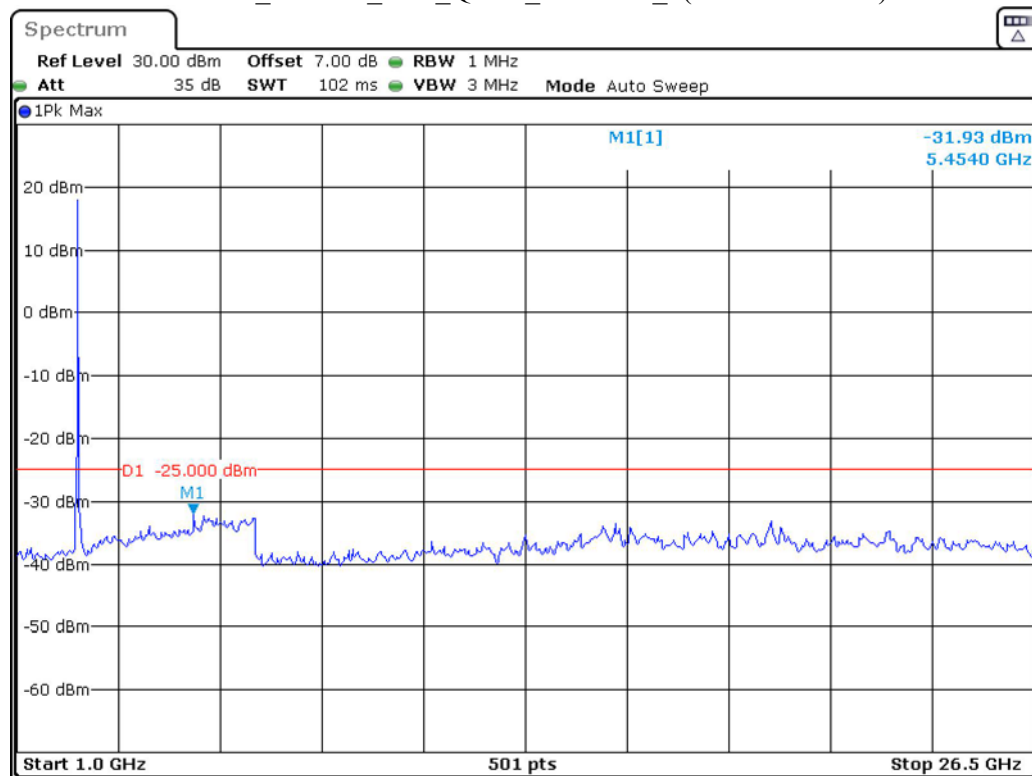
Band 41_20 MHz_Low_QPSK_RB100#0_2(1GHz-26.5GHz)
