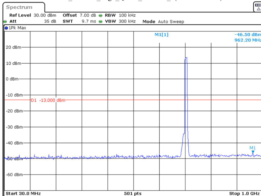
Band 12_10 MHz_High_QPSK_RB50#0_1(30MHz-1GHz)
