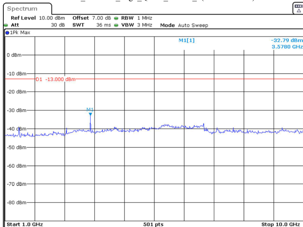
Band 12_1.4 MHz_High_QPSK_RB6#0_2(1GHz-10GHz)
