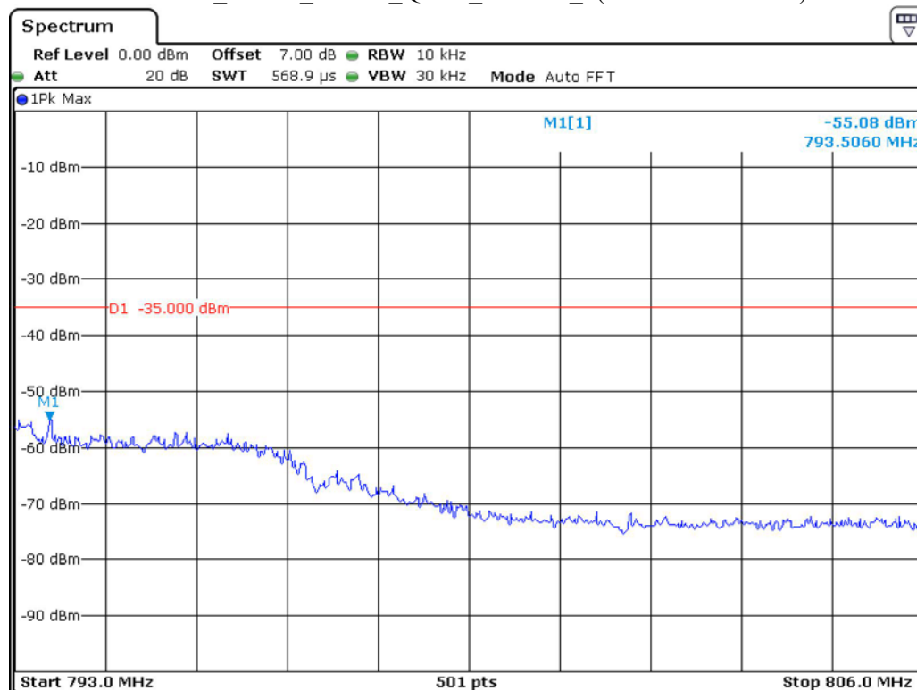
Band 13_5 MHz_Middle_QPSK_RB25#0_3(793MHz-806MHz)
