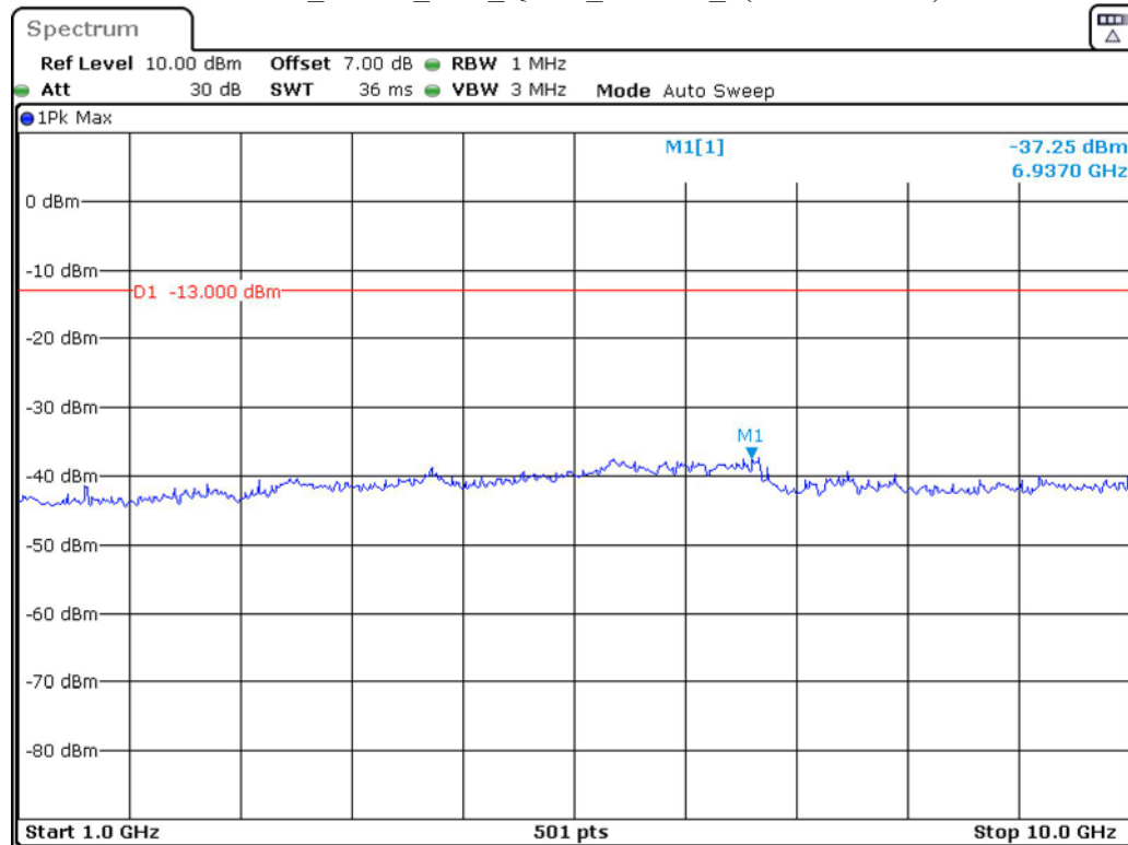
Band 13_5 MHz_Low_QPSK_RB25#0_2(1GHz-10GHz)
