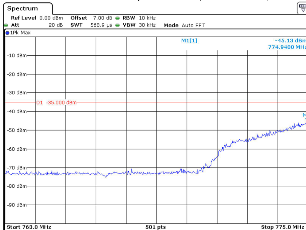
Band 13_5 MHz_Middle_QPSK_RB25#0_2(763MHz-775MHz)
