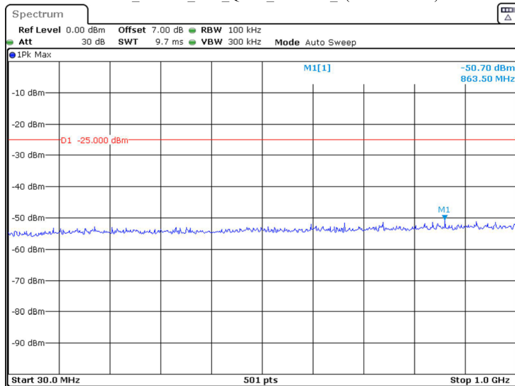
Band 41_20 MHz_Low_QPSK_RB100#0_1(30MHz-1GHz)
