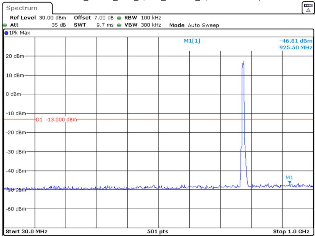
Band 13_5 MHz_Low_QPSK_RB25#0_1(30MHz-1GHz)
