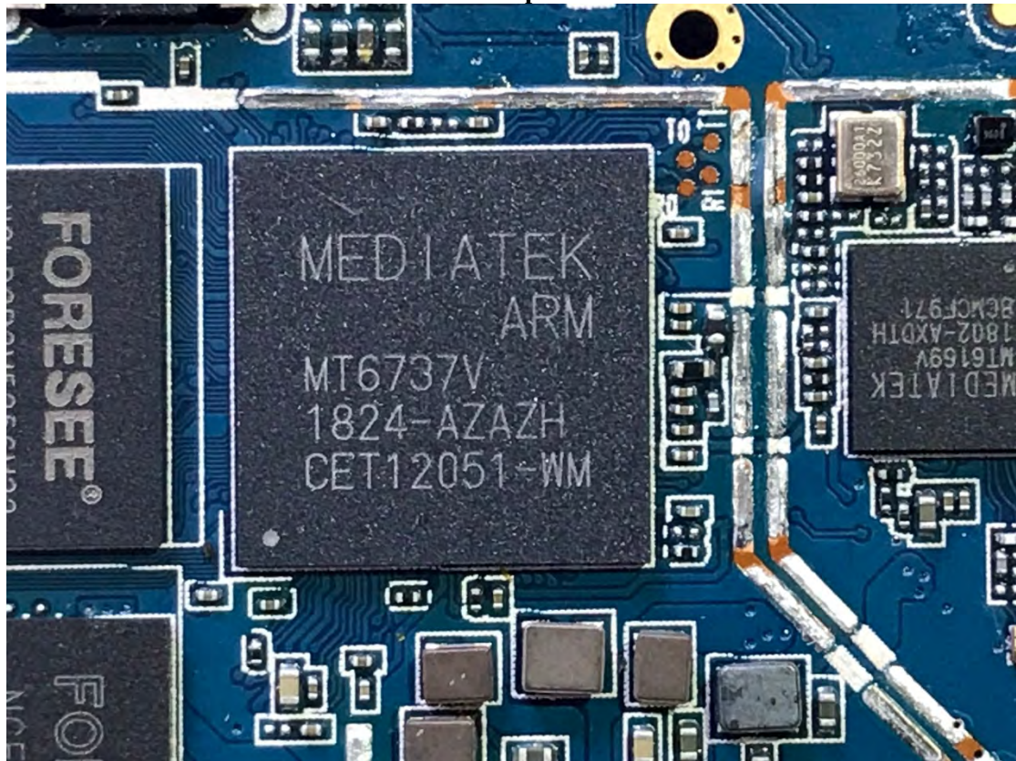
Main Chip View
